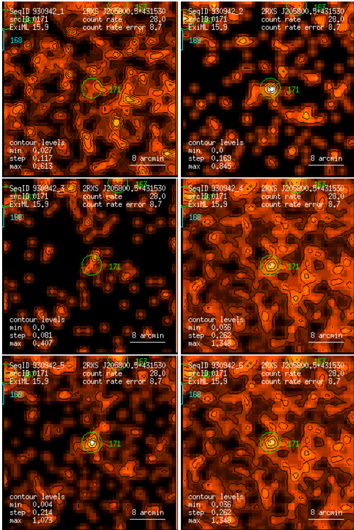
Figure 171: RASS 930942: detection 0171: band rate images, Gaussian filter: (1) PSPC channels 11 – 41, (2) 52 – 90, (3) 91 – 201, (4) 11 – 235, (5) 52 – 201, (6) 11 – 201. Broad band rates in counts/ks. Band rate contour levels in counts/ks/arcmin 2 .
