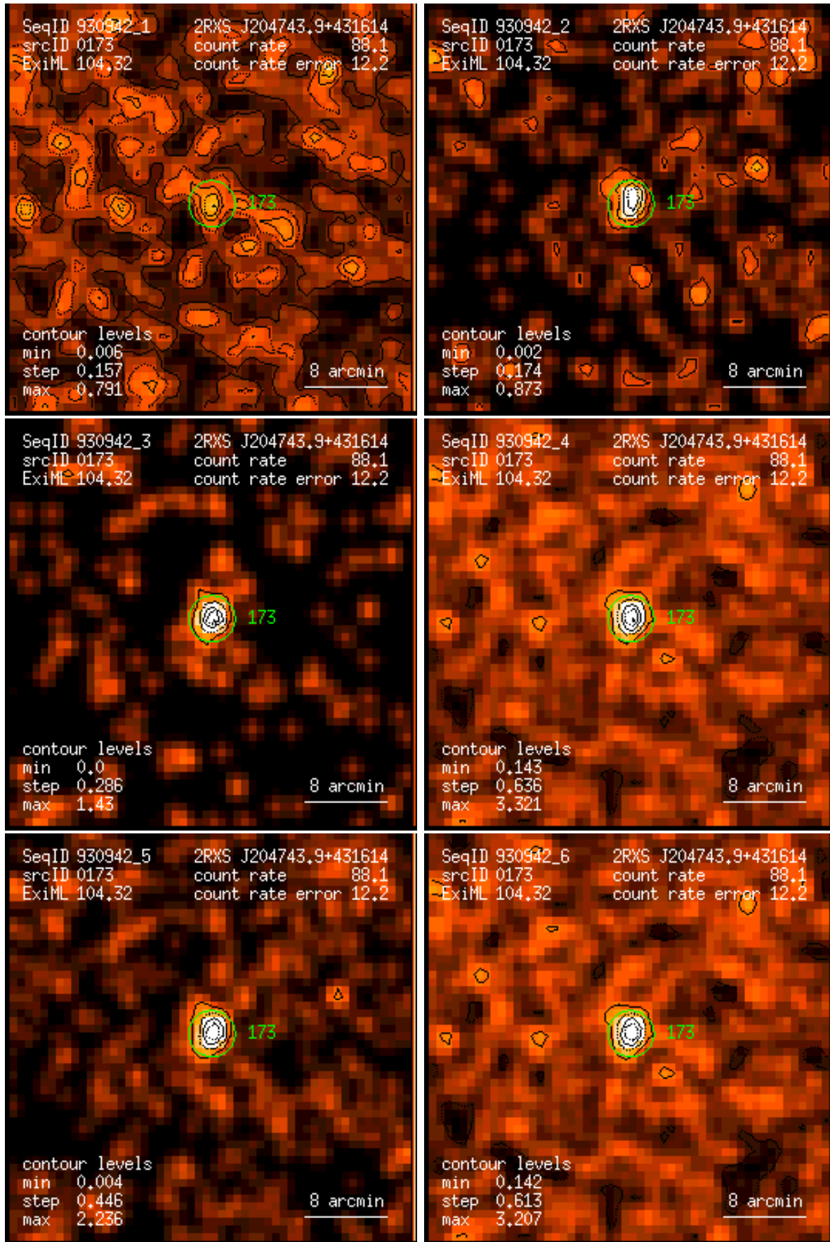
Figure 173: RASS 930942: detection 0173: band rate images, Gaussian filter: (1) PSPC channels 11 – 41, (2) 52 – 90, (3) 91 – 201, (4) 11 – 235, (5) 52 – 201, (6) 11 – 201. Broad band rates in counts/ks. Band rate contour levels in counts/ks/arcmin 2 .
