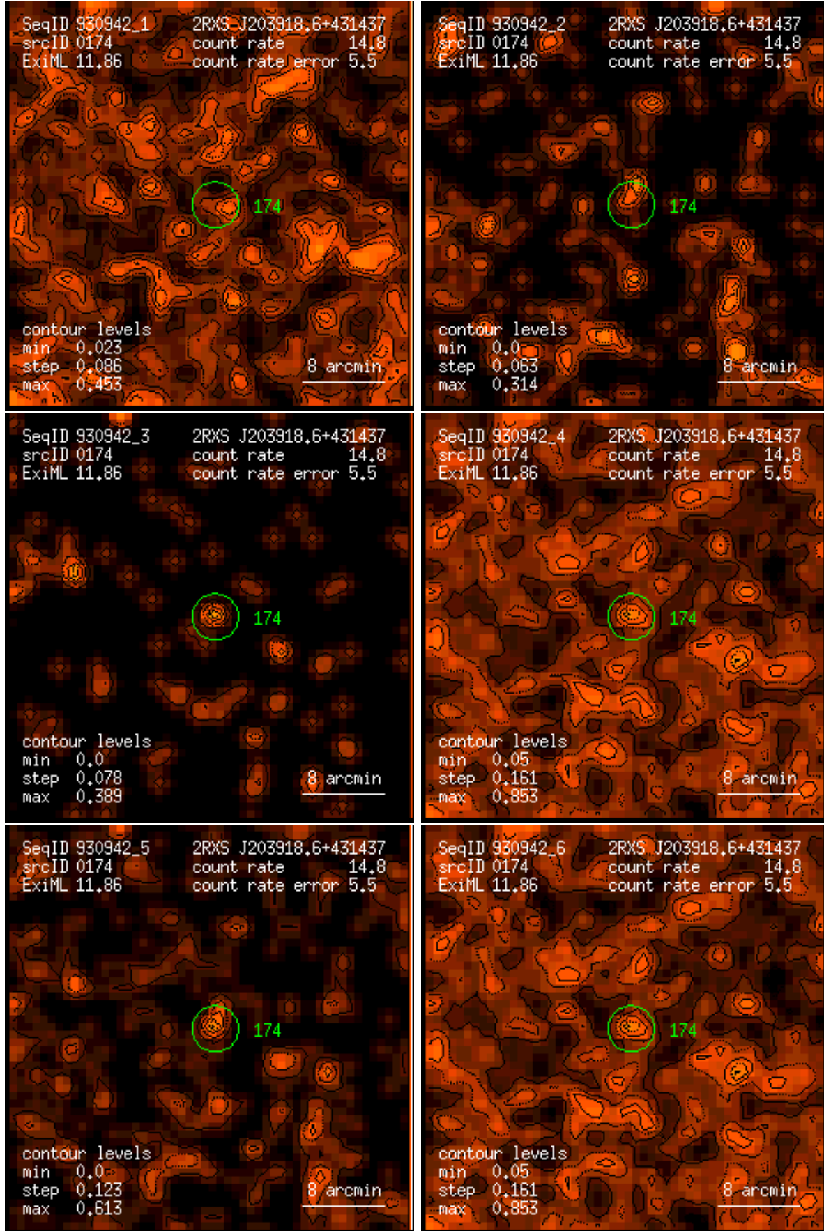
Figure 174: RASS 930942: detection 0174: band rate images, Gaussian filter: (1) PSPC channels 11 – 41, (2) 52 – 90, (3) 91 – 201, (4) 11 – 235, (5) 52 – 201, (6) 11 – 201. Broad band rates in counts/ks. Band rate contour levels in counts/ks/arcmin 2 .
