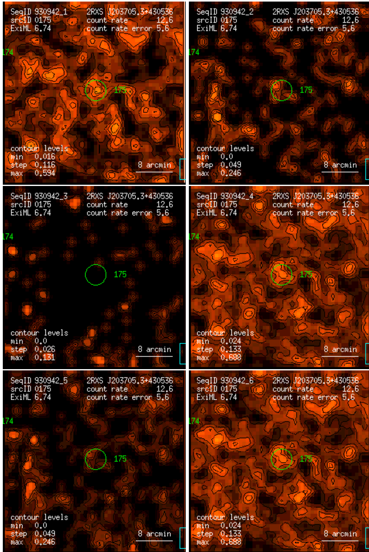
Figure 175: RASS 930942: detection 0175: band rate images, Gaussian filter: (1) PSPC channels 11 – 41, (2) 52 – 90, (3) 91 – 201, (4) 11 – 235, (5) 52 – 201, (6) 11 – 201. Broad band rates in counts/ks. Band rate contour levels in counts/ks/arcmin 2 .
