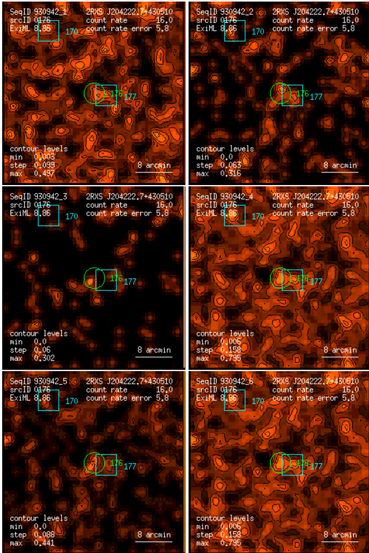
Figure 176: RASS 930942: detection 0176: band rate images, Gaussian filter: (1) PSPC channels 11 – 41, (2) 52 – 90, (3) 91 – 201, (4) 11 – 235, (5) 52 – 201, (6) 11 – 201. Broad band rates in counts/ks. Band rate contour levels in counts/ks/arcmin 2 .
