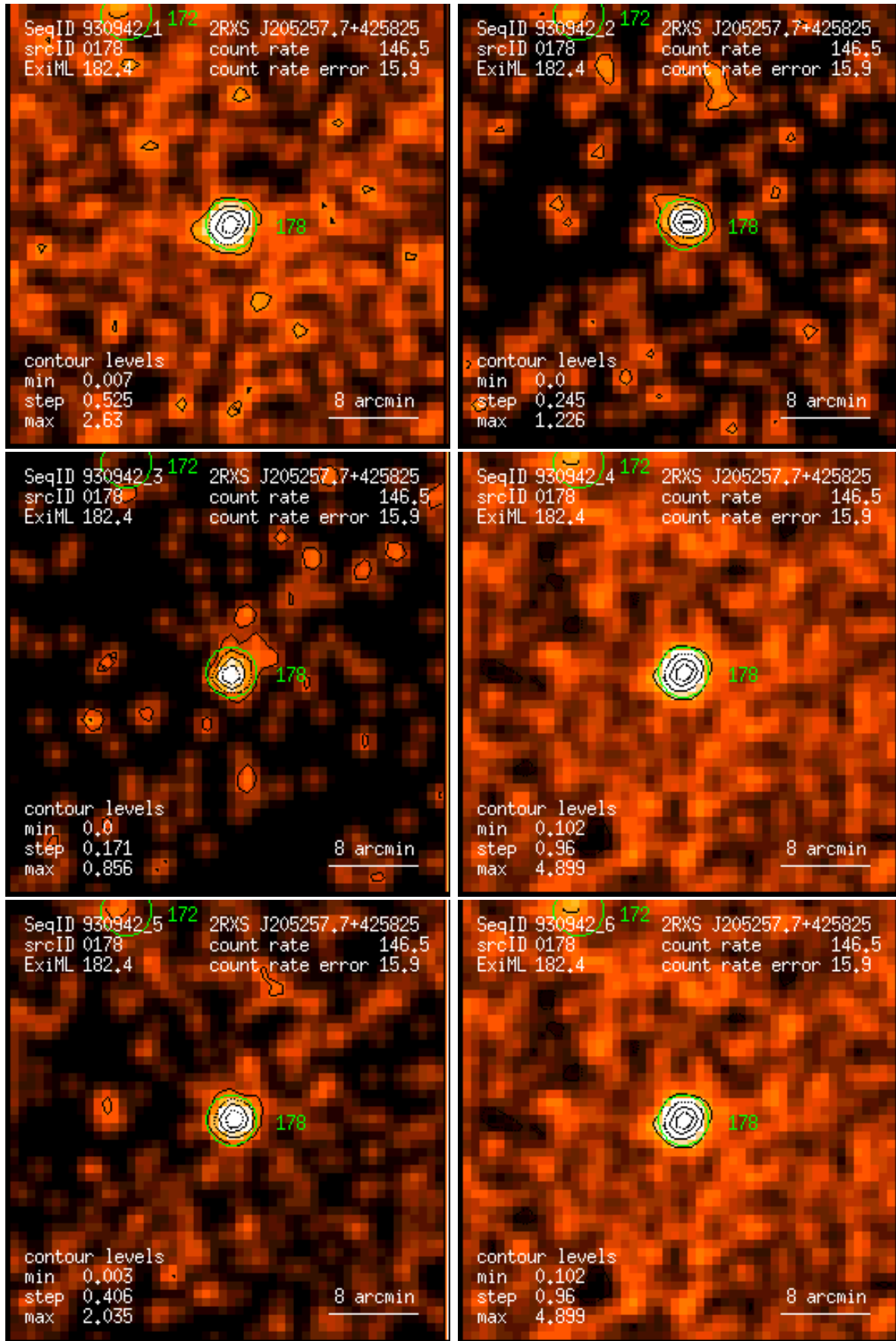
Figure 178: RASS 930942: detection 0178: band rate images, Gaussian filter: (1) PSPC channels 11 – 41, (2) 52 – 90, (3) 91 – 201, (4) 11 – 235, (5) 52 – 201, (6) 11 – 201. Broad band rates in counts/ks. Band rate contour levels in counts/ks/arcmin 2 .
