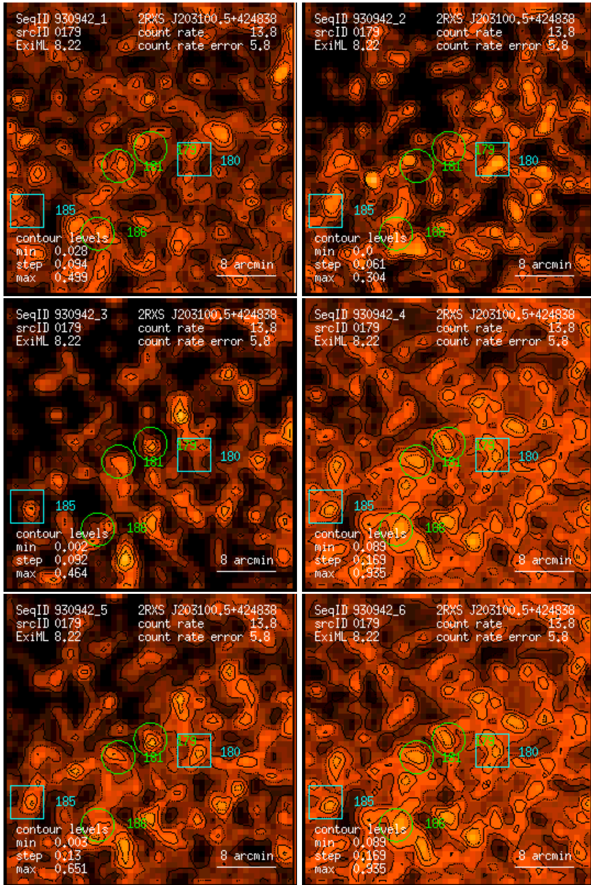
Figure 179: RASS 930942: detection 0179: band rate images, Gaussian filter: (1) PSPC channels 11 – 41, (2) 52 – 90, (3) 91 – 201, (4) 11 – 235, (5) 52 – 201, (6) 11 – 201. Broad band rates in counts/ks. Band rate contour levels in counts/ks/arcmin 2 .
