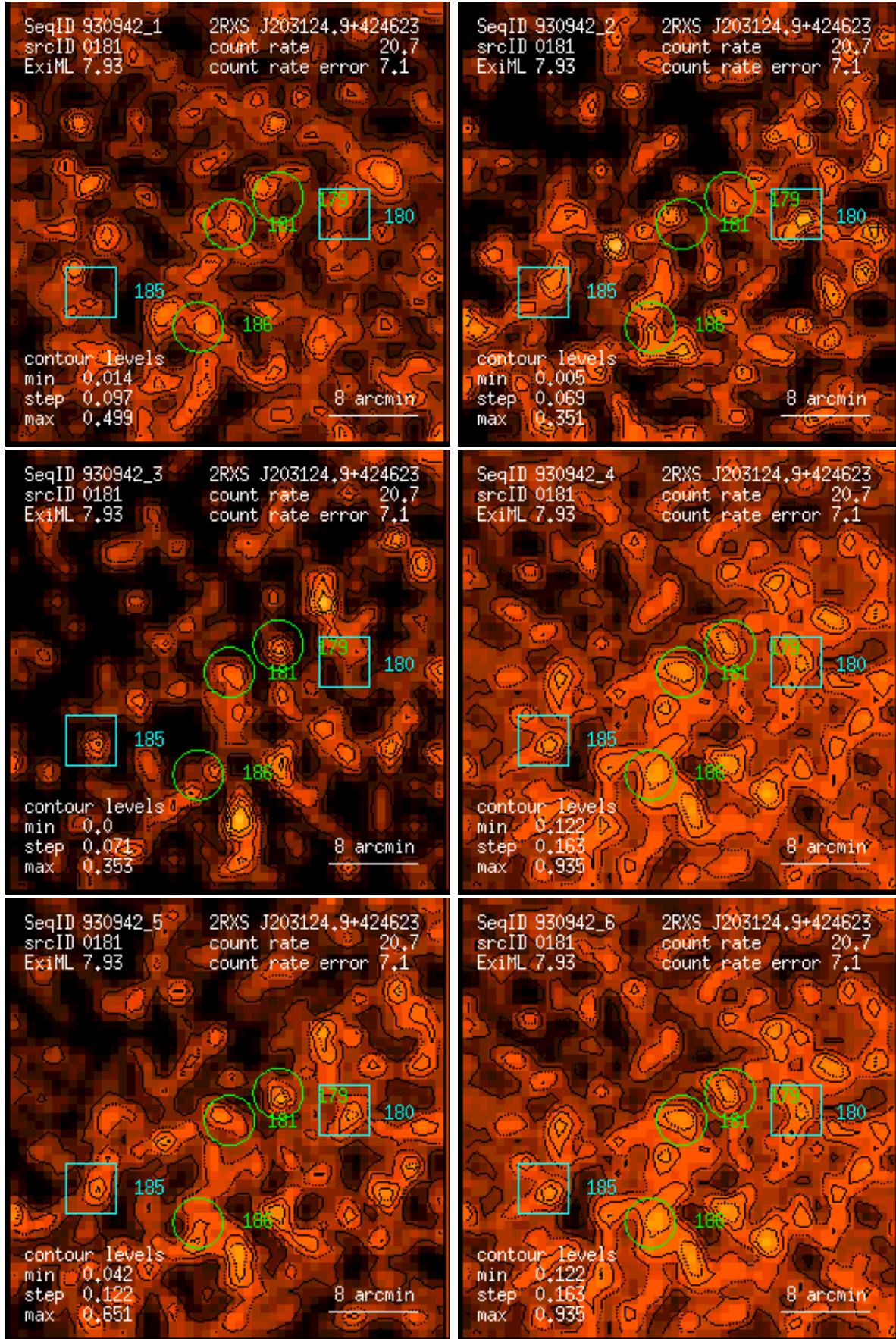
Figure 181: RASS 930942: detection 0181: band rate images, Gaussian filter: (1) PSPC channels 11 – 41, (2) 52 – 90, (3) 91 – 201, (4) 11 – 235, (5) 52 – 201, (6) 11 – 201. Broad band rates in counts/ks. Band rate contour levels in counts/ks/arcmin 2 .
