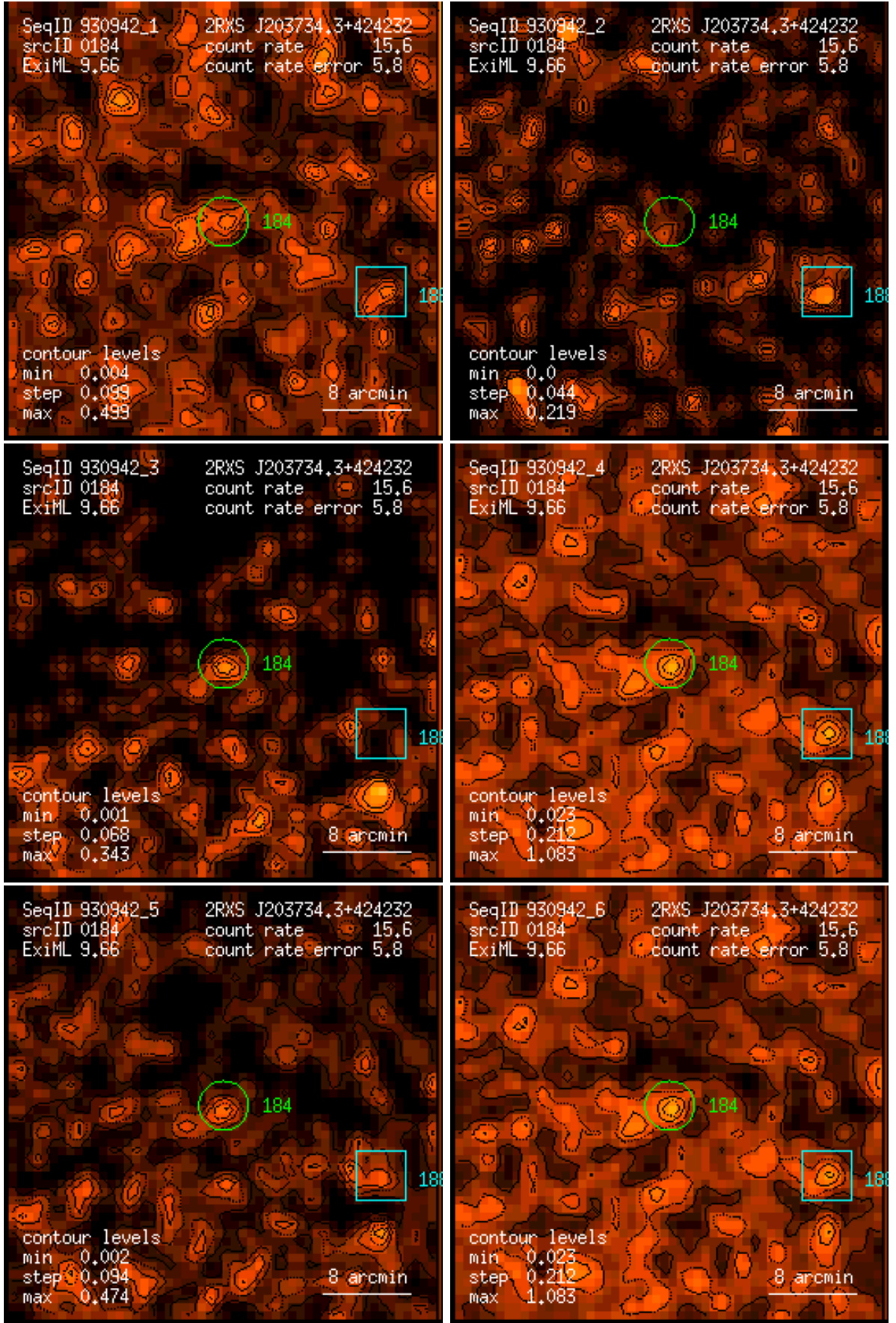
Figure 184: RASS 930942: detection 0184: band rate images, Gaussian filter: (1) PSPC channels 11 – 41, (2) 52 – 90, (3) 91 – 201, (4) 11 – 235, (5) 52 – 201, (6) 11 – 201. Broad band rates in counts/ks. Band rate contour levels in counts/ks/arcmin 2 .
