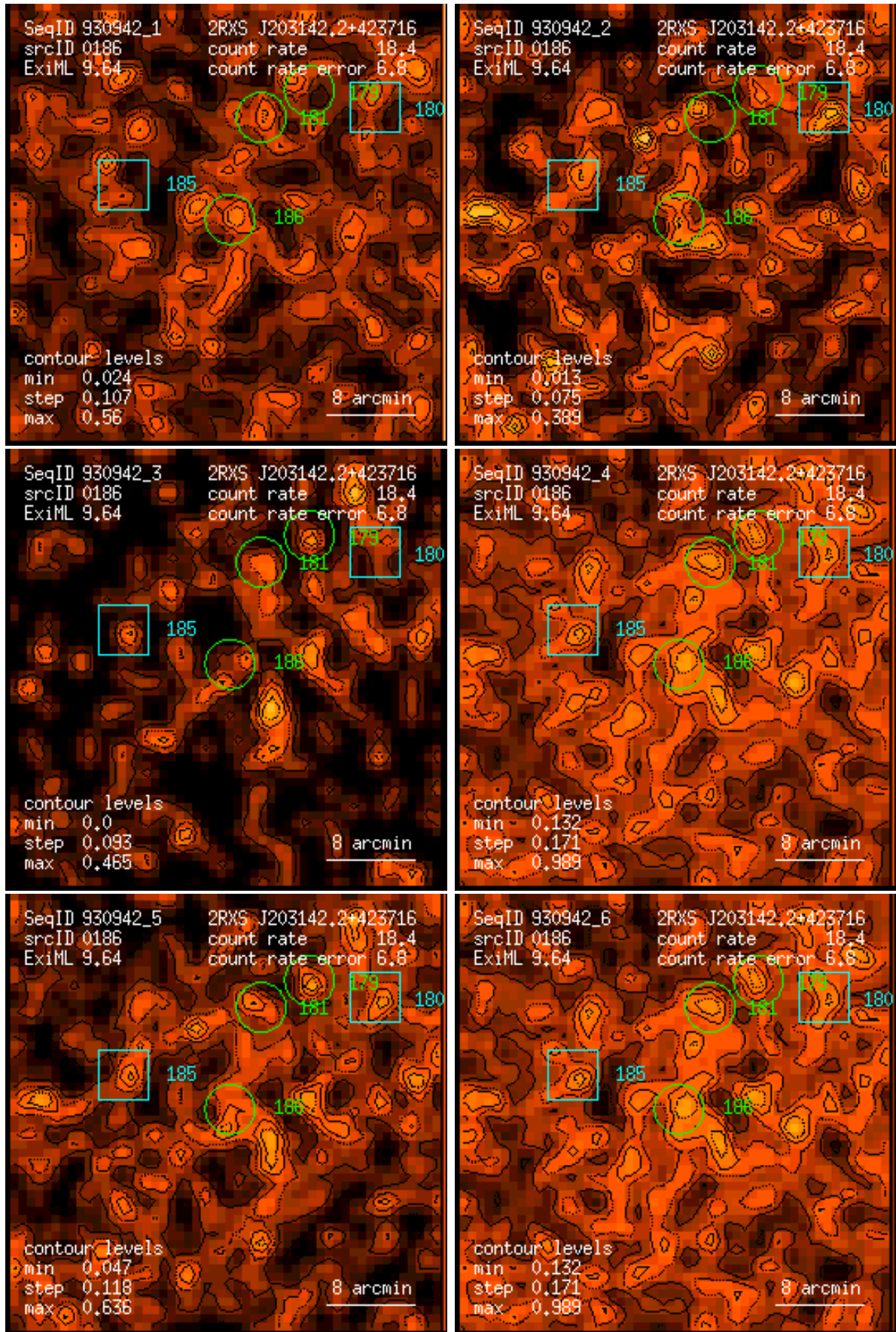
Figure 186: RASS 930942: detection 0186: band rate images, Gaussian filter: (1) PSPC channels 11 – 41, (2) 52 – 90, (3) 91 – 201, (4) 11 – 235, (5) 52 – 201, (6) 11 – 201. Broad band rates in counts/ks. Band rate contour levels in counts/ks/arcmin 2 .
