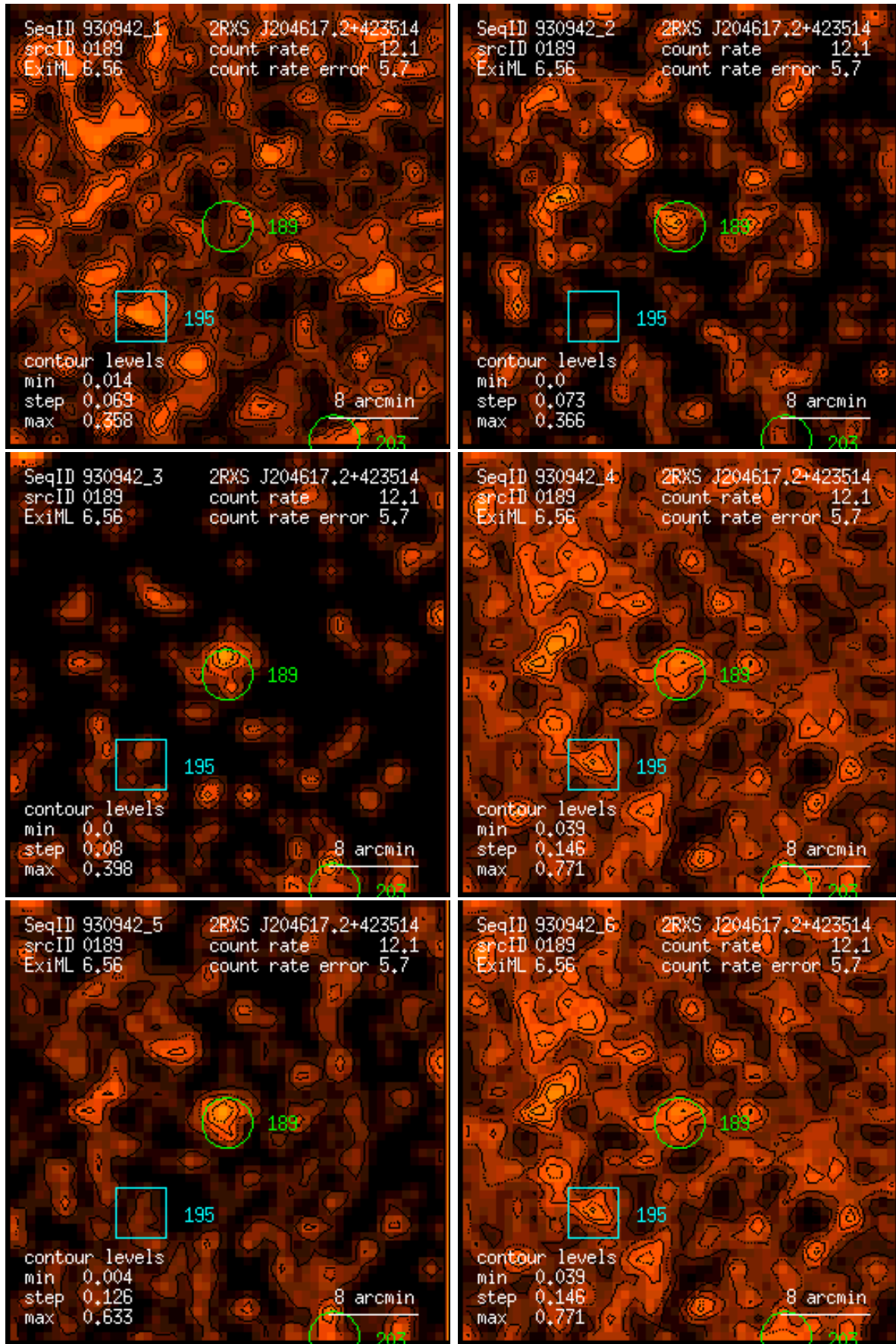
Figure 189: RASS 930942: detection 0189: band rate images, Gaussian filter: (1) PSPC channels 11 – 41, (2) 52 – 90, (3) 91 – 201, (4) 11 – 235, (5) 52 – 201, (6) 11 – 201. Broad band rates in counts/ks. Band rate contour levels in counts/ks/arcmin 2 .
