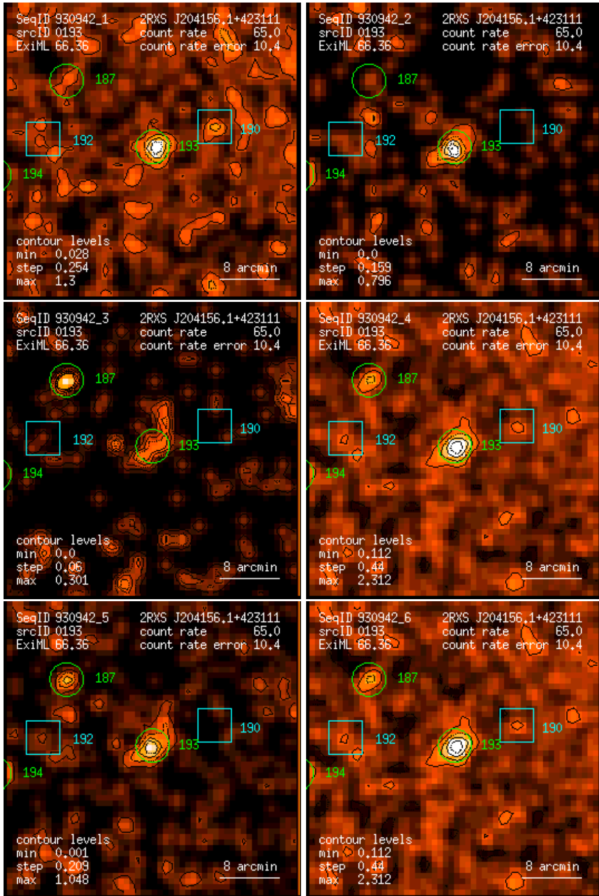
Figure 193: RASS 930942: detection 0193: band rate images, Gaussian filter: (1) PSPC channels 11 – 41, (2) 52 – 90, (3) 91 – 201, (4) 11 – 235, (5) 52 – 201, (6) 11 – 201. Broad band rates in counts/ks. Band rate contour levels in counts/ks/arcmin 2 .
