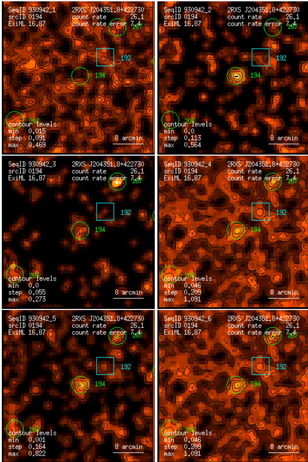
Figure 194: RASS 930942: detection 0194: band rate images, Gaussian filter: (1) PSPC channels 11 – 41, (2) 52 – 90, (3) 91 – 201, (4) 11 – 235, (5) 52 – 201, (6) 11 – 201. Broad band rates in counts/ks. Band rate contour levels in counts/ks/arcmin 2 .
