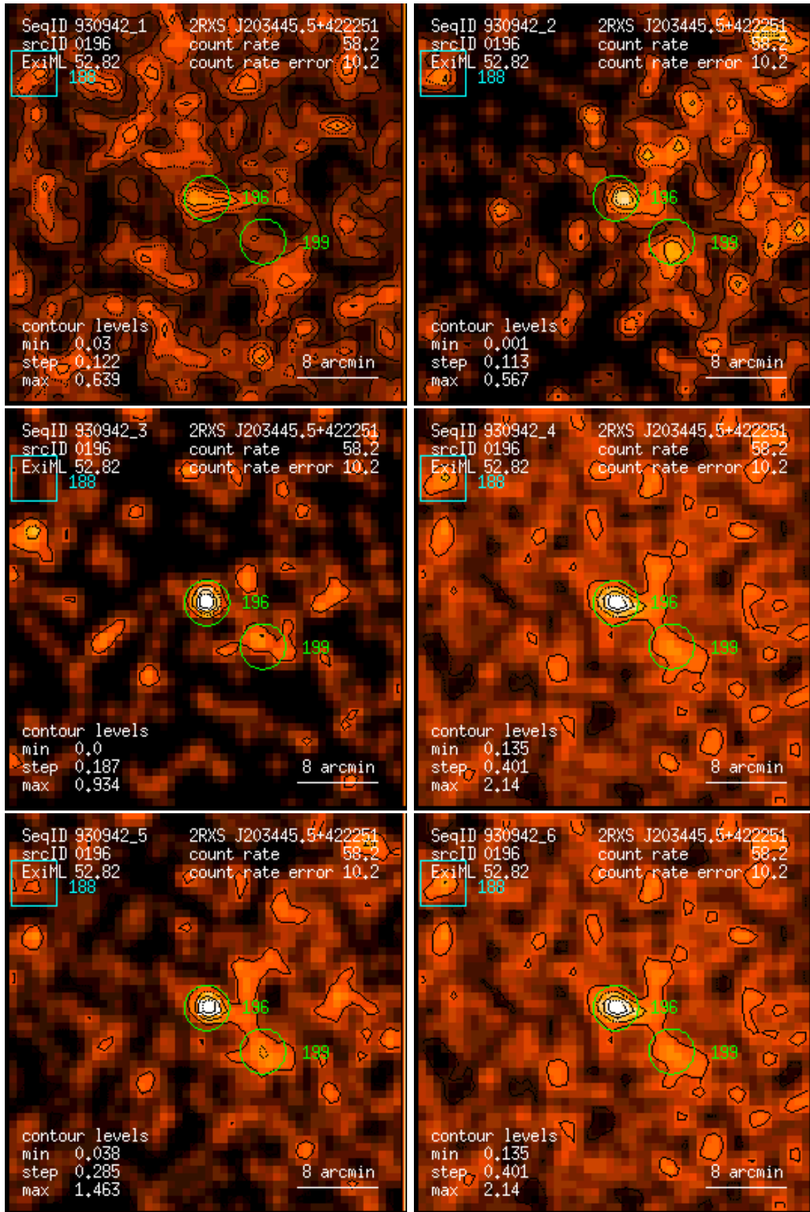
Figure 196: RASS 930942: detection 0196: band rate images, Gaussian filter: (1) PSPC channels 11 – 41, (2) 52 – 90, (3) 91 – 201, (4) 11 – 235, (5) 52 – 201, (6) 11 – 201. Broad band rates in counts/ks. Band rate contour levels in counts/ks/arcmin 2 .
