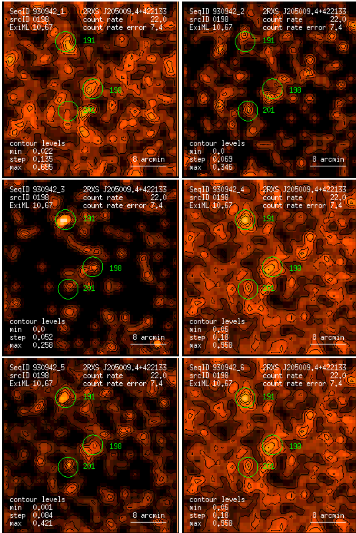
Figure 198: RASS 930942: detection 0198: band rate images, Gaussian filter: (1) PSPC channels 11 – 41, (2) 52 – 90, (3) 91 – 201, (4) 11 – 235, (5) 52 – 201, (6) 11 – 201. Broad band rates in counts/ks. Band rate contour levels in counts/ks/arcmin 2 .
