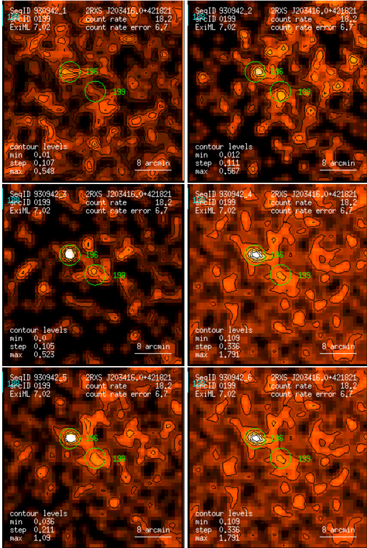
Figure 199: RASS 930942: detection 0199: band rate images, Gaussian filter: (1) PSPC channels 11 – 41, (2) 52 – 90, (3) 91 – 201, (4) 11 – 235, (5) 52 – 201, (6) 11 – 201. Broad band rates in counts/ks. Band rate contour levels in counts/ks/arcmin 2 .
