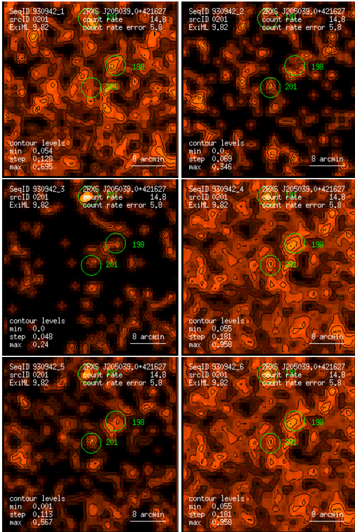
Figure 201: RASS 930942: detection 0201: band rate images, Gaussian filter: (1) PSPC channels 11 – 41, (2) 52 – 90, (3) 91 – 201, (4) 11 – 235, (5) 52 – 201, (6) 11 – 201. Broad band rates in counts/ks. Band rate contour levels in counts/ks/arcmin 2 .
