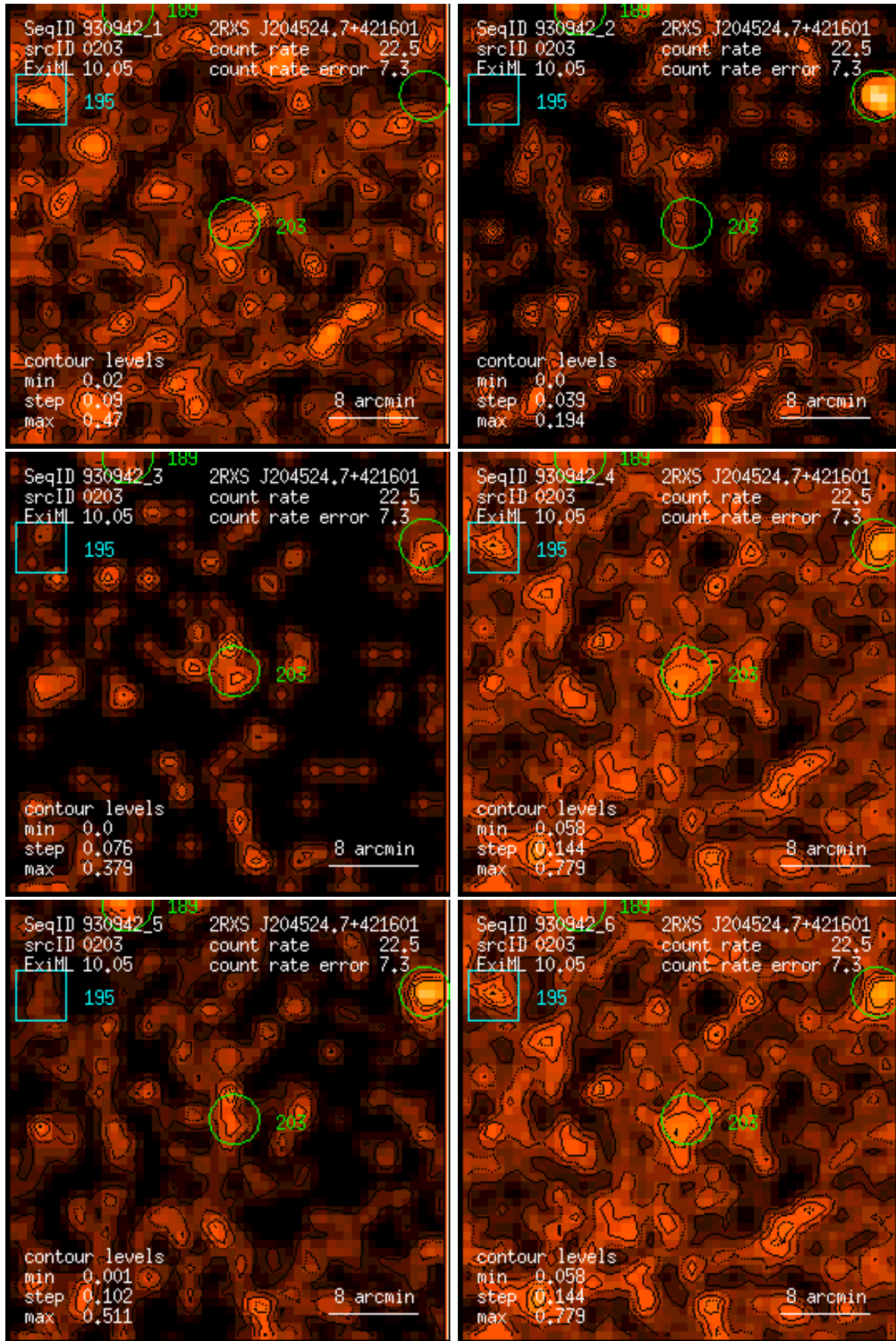
Figure 203: RASS 930942: detection 0203: band rate images, Gaussian filter: (1) PSPC channels 11 – 41, (2) 52 – 90, (3) 91 – 201, (4) 11 – 235, (5) 52 – 201, (6) 11 – 201. Broad band rates in counts/ks. Band rate contour levels in counts/ks/arcmin 2 .
