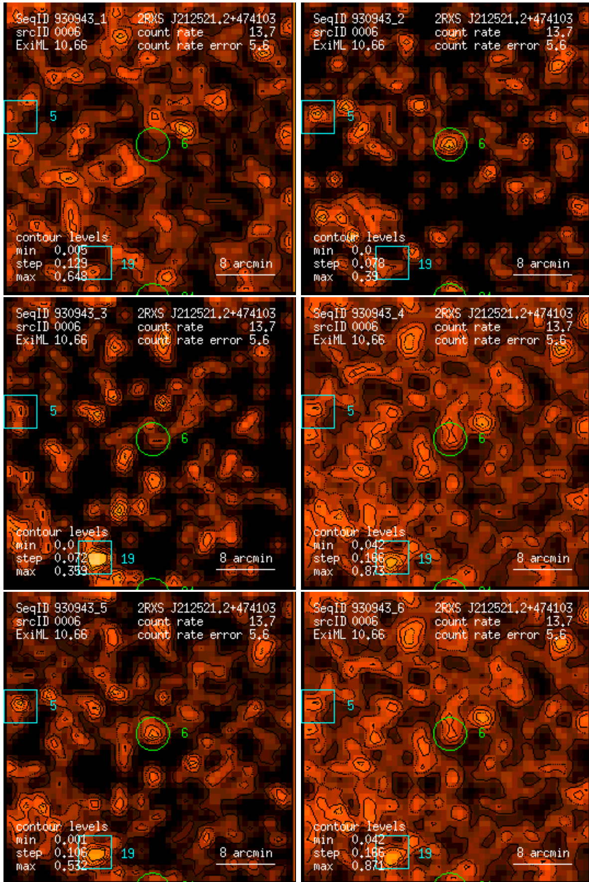
Figure 6: RASS 930943: detection 0006: band rate images, Gaussian filter: (1) PSPC channels 11 – 41, (2) 52 – 90, (3) 91 – 201, (4) 11 – 235, (5) 52 – 201, (6) 11 – 201. Broad band rates in counts/ks. Band rate contour levels in counts/ks/arcmin 2 .
