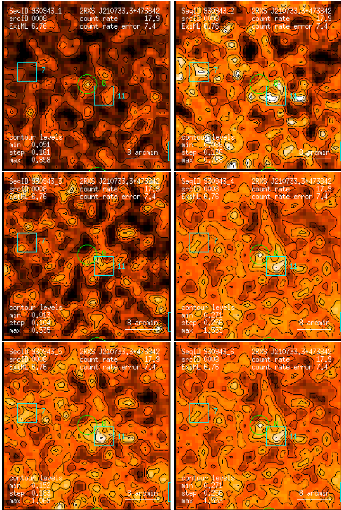
Figure 8: RASS 930943: detection 0008: band rate images, Gaussian filter: (1) PSPC channels 11 – 41, (2) 52 – 90, (3) 91 – 201, (4) 11 – 235, (5) 52 – 201, (6) 11 – 201. Broad band rates in counts/ks. Band rate contour levels in counts/ks/arcmin 2 .
