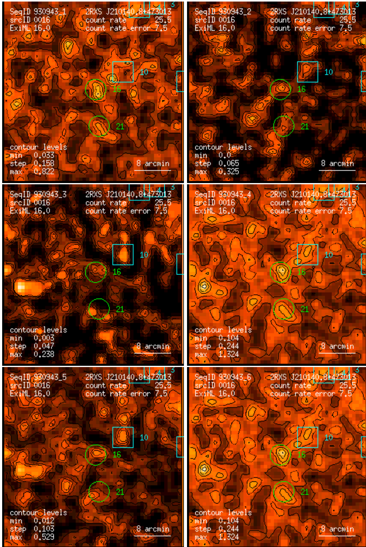
Figure 16: RASS 930943: detection 0016: band rate images, Gaussian filter: (1) PSPC channels 11 – 41, (2) 52 – 90, (3) 91 – 201, (4) 11 – 235, (5) 52 – 201, (6) 11 – 201. Broad band rates in counts/ks. Band rate contour levels in counts/ks/arcmin 2 .
