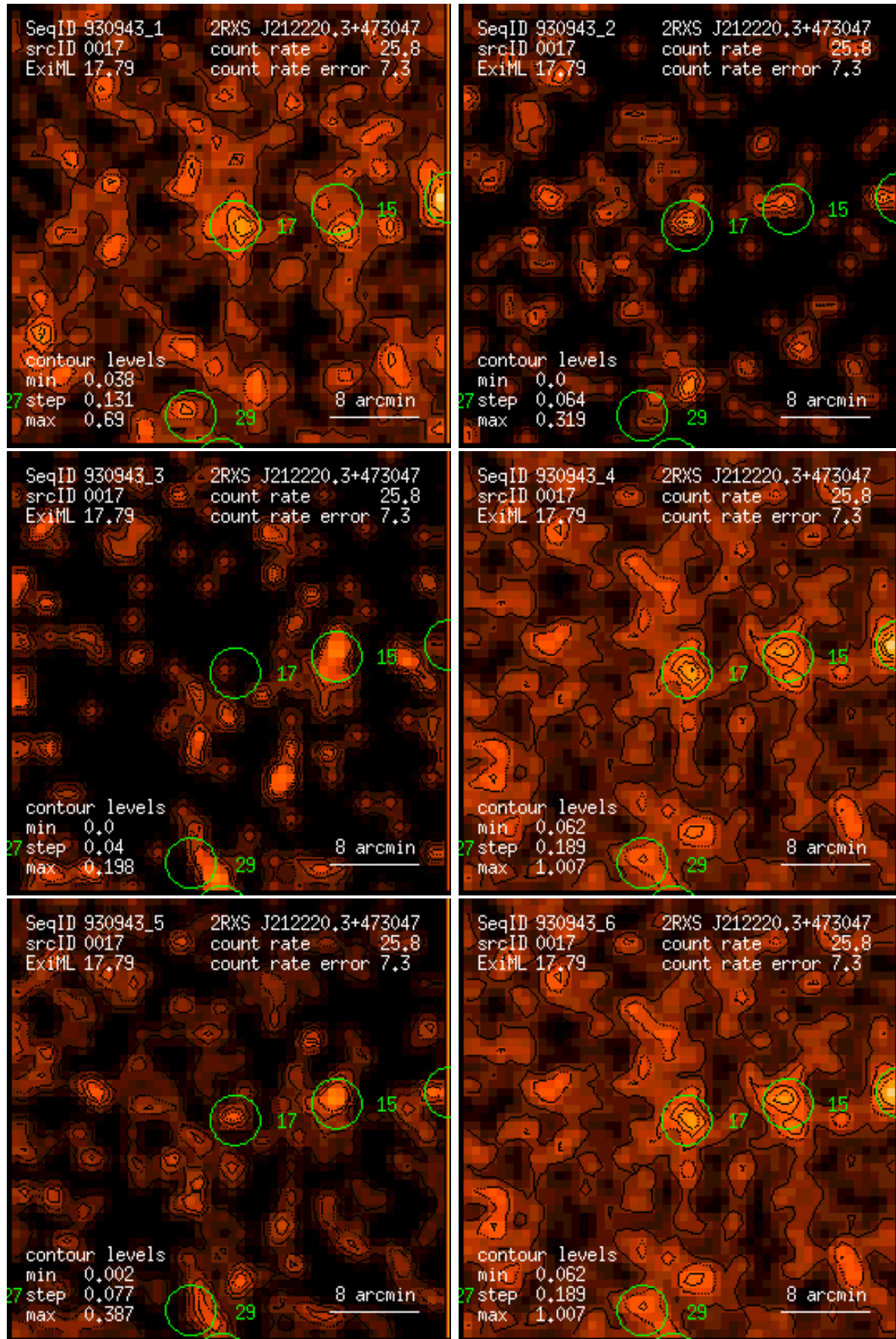
Figure 17: RASS 930943: detection 0017: band rate images, Gaussian filter: (1) PSPC channels 11 – 41, (2) 52 – 90, (3) 91 – 201, (4) 11 – 235, (5) 52 – 201, (6) 11 – 201. Broad band rates in counts/ks. Band rate contour levels in counts/ks/arcmin 2 .
