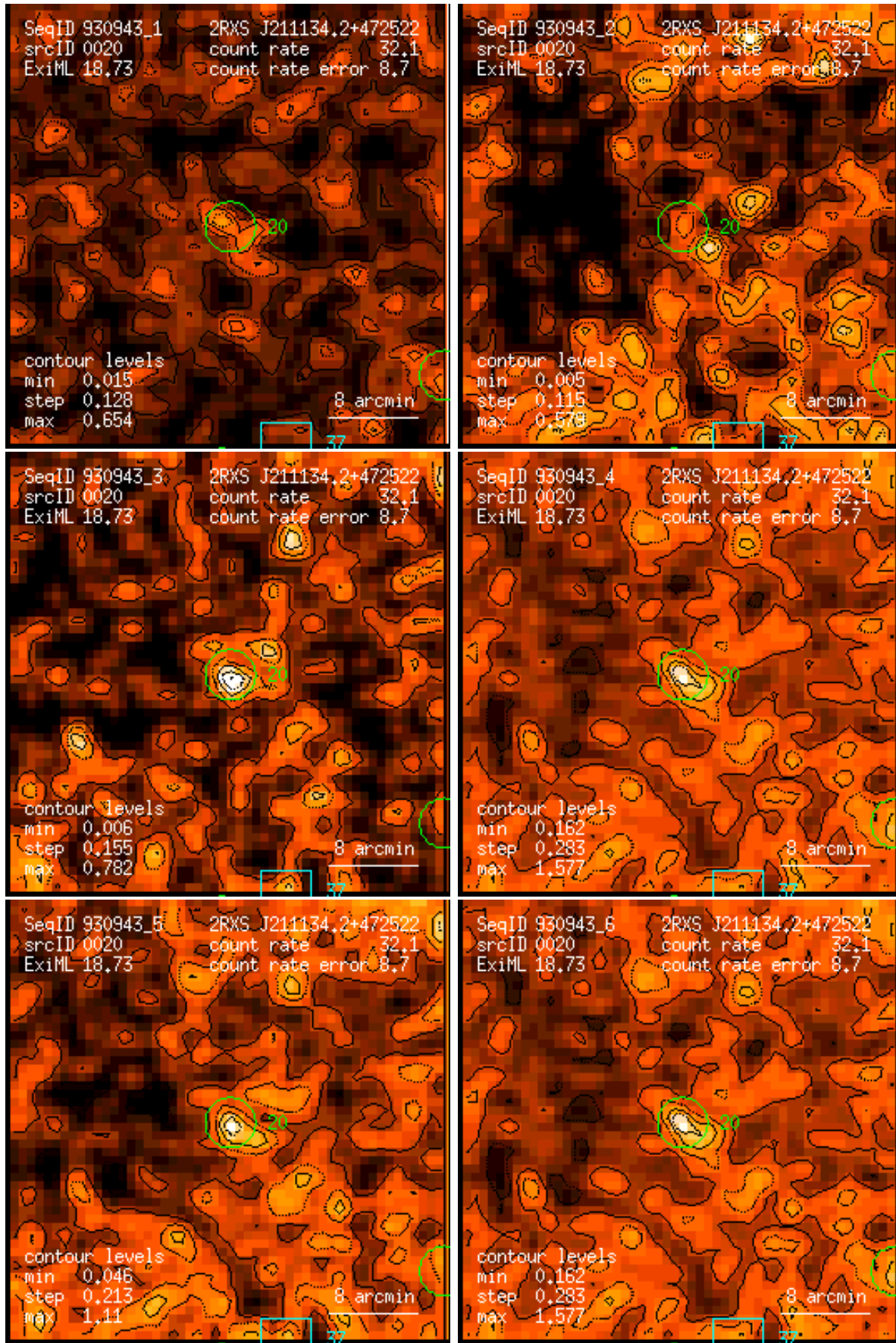
Figure 20: RASS 930943: detection 0020: band rate images, Gaussian filter: (1) PSPC channels 11 – 41, (2) 52 – 90, (3) 91 – 201, (4) 11 – 235, (5) 52 – 201, (6) 11 – 201. Broad band rates in counts/ks. Band rate contour levels in counts/ks/arcmin 2 .
