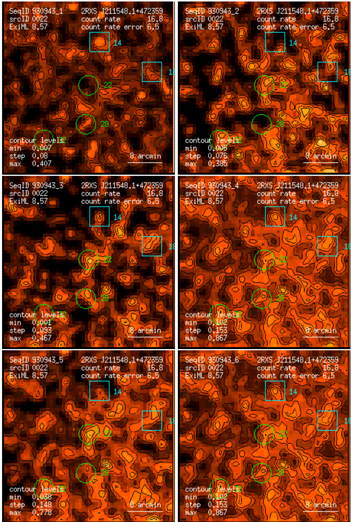
Figure 22: RASS 930943: detection 0022: band rate images, Gaussian filter: (1) PSPC channels 11 – 41, (2) 52 – 90, (3) 91 – 201, (4) 11 – 235, (5) 52 – 201, (6) 11 – 201. Broad band rates in counts/ks. Band rate contour levels in counts/ks/arcmin 2 .
