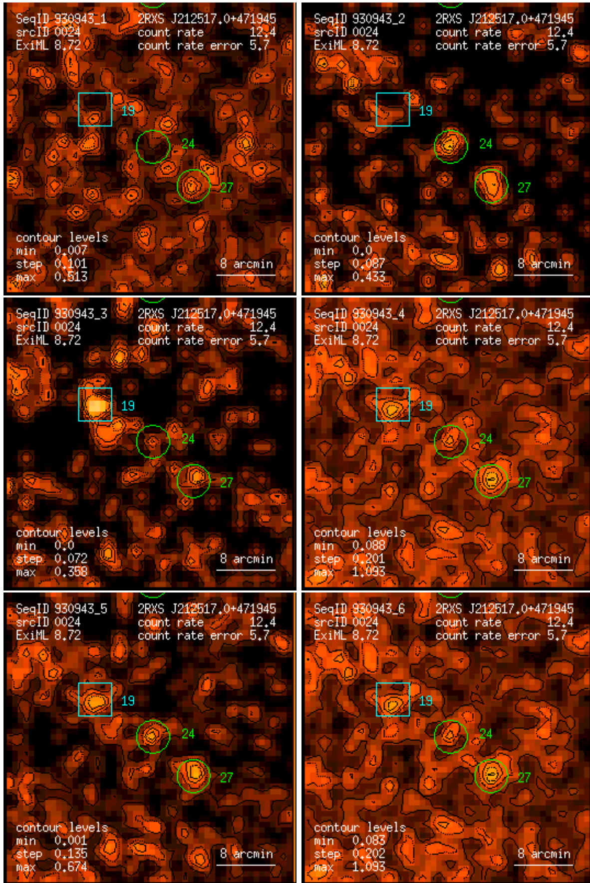
Figure 24: RASS 930943: detection 0024: band rate images, Gaussian filter: (1) PSPC channels 11 – 41, (2) 52 – 90, (3) 91 – 201, (4) 11 – 235, (5) 52 – 201, (6) 11 – 201. Broad band rates in counts/ks. Band rate contour levels in counts/ks/arcmin 2 .
