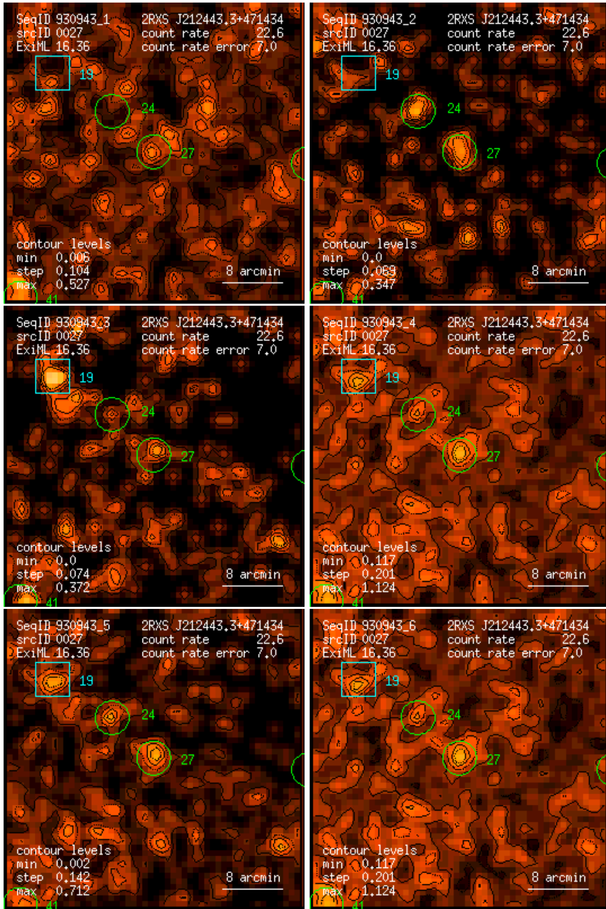
Figure 27: RASS 930943: detection 0027: band rate images, Gaussian filter: (1) PSPC channels 11 – 41, (2) 52 – 90, (3) 91 – 201, (4) 11 – 235, (5) 52 – 201, (6) 11 – 201. Broad band rates in counts/ks. Band rate contour levels in counts/ks/arcmin 2 .
