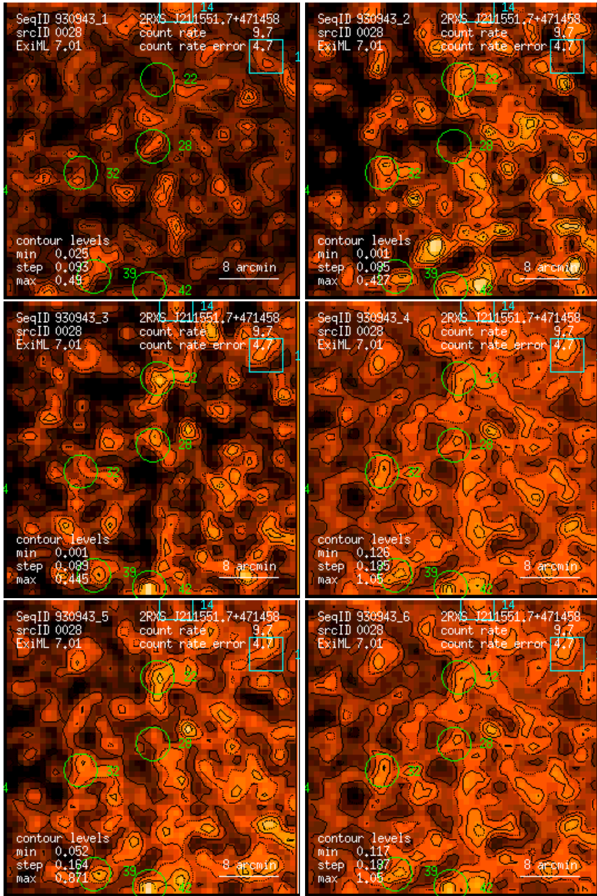
Figure 28: RASS 930943: detection 0028: band rate images, Gaussian filter: (1) PSPC channels 11 – 41, (2) 52 – 90, (3) 91 – 201, (4) 11 – 235, (5) 52 – 201, (6) 11 – 201. Broad band rates in counts/ks. Band rate contour levels in counts/ks/arcmin 2 .
