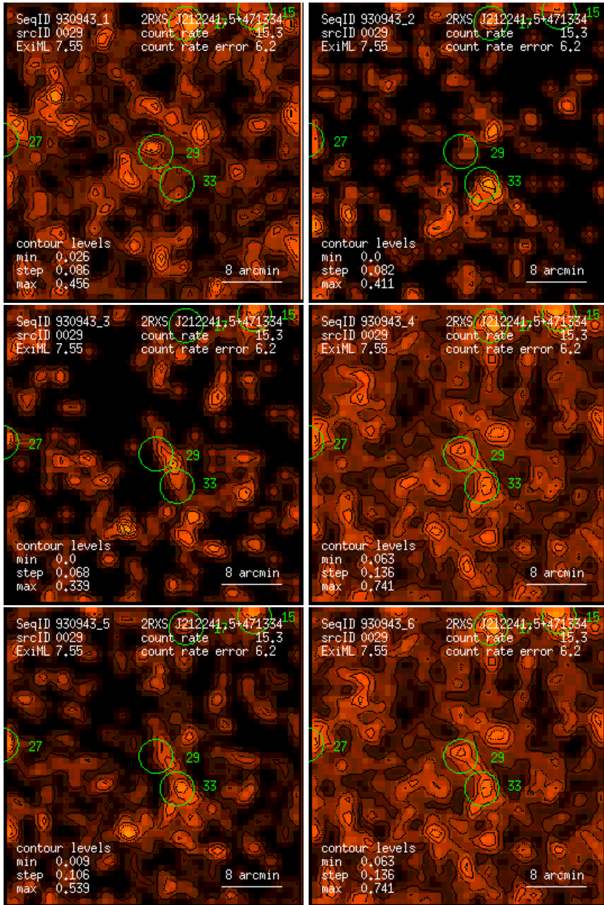
Figure 29: RASS 930943: detection 0029: band rate images, Gaussian filter: (1) PSPC channels 11 – 41, (2) 52 – 90, (3) 91 – 201, (4) 11 – 235, (5) 52 – 201, (6) 11 – 201. Broad band rates in counts/ks. Band rate contour levels in counts/ks/arcmin 2 .
