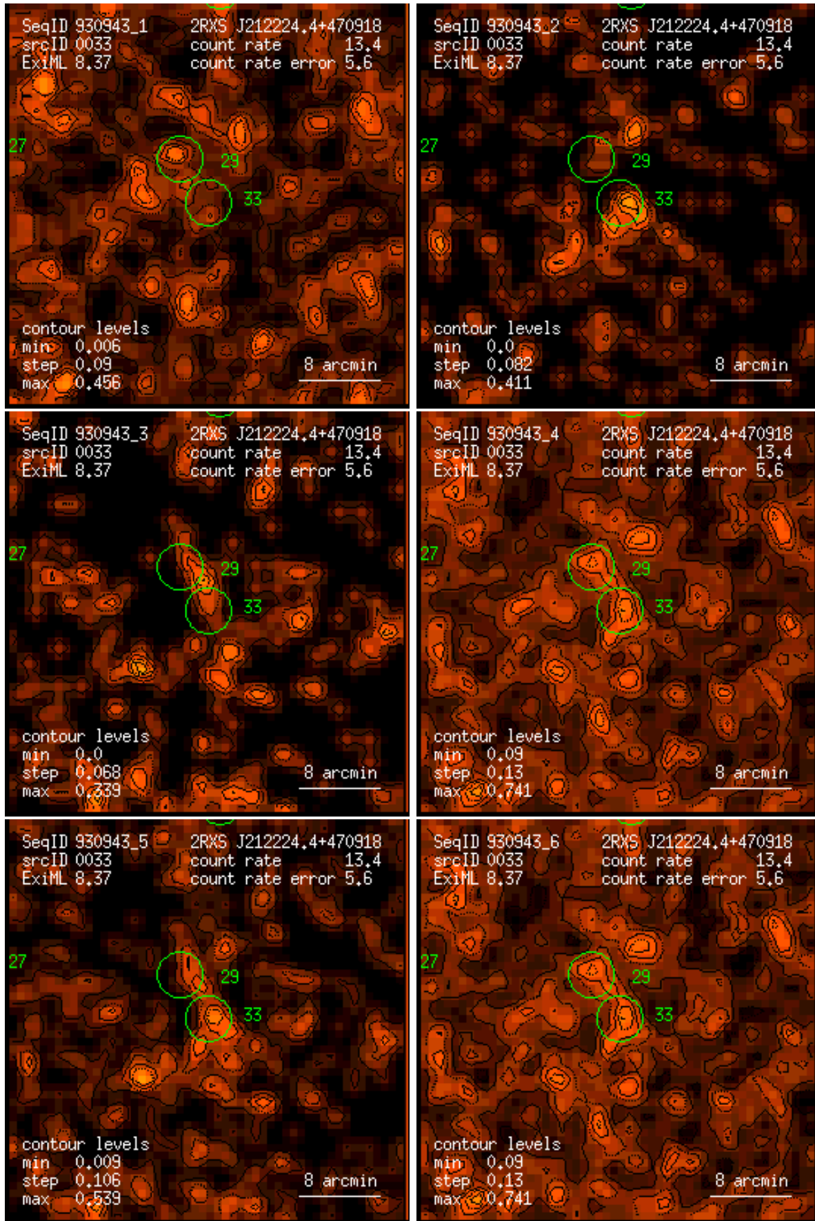
Figure 33: RASS 930943: detection 0033: band rate images, Gaussian filter: (1) PSPC channels 11 – 41, (2) 52 – 90, (3) 91 – 201, (4) 11 – 235, (5) 52 – 201, (6) 11 – 201. Broad band rates in counts/ks. Band rate contour levels in counts/ks/arcmin 2 .
