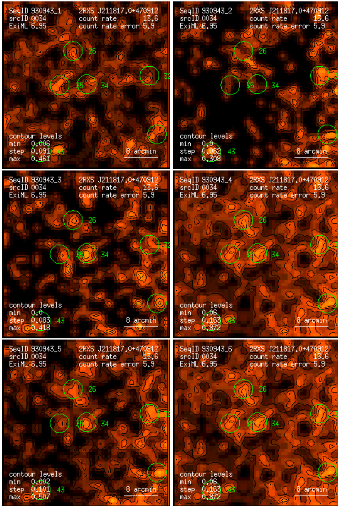
Figure 34: RASS 930943: detection 0034: band rate images, Gaussian filter: (1) PSPC channels 11 – 41, (2) 52 – 90, (3) 91 – 201, (4) 11 – 235, (5) 52 – 201, (6) 11 – 201. Broad band rates in counts/ks. Band rate contour levels in counts/ks/arcmin 2 .
