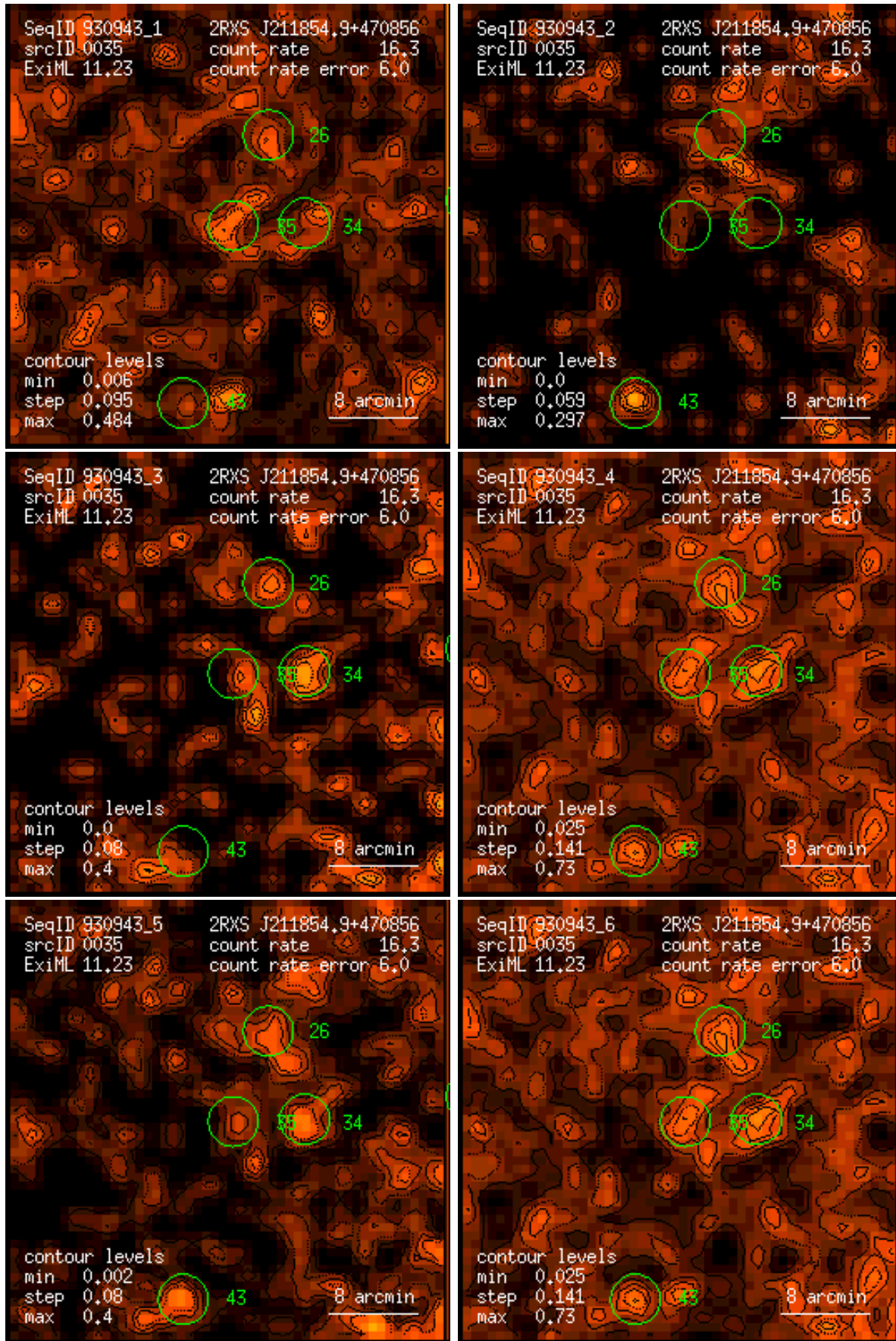
Figure 35: RASS 930943: detection 0035: band rate images, Gaussian filter: (1) PSPC channels 11 – 41, (2) 52 – 90, (3) 91 – 201, (4) 11 – 235, (5) 52 – 201, (6) 11 – 201. Broad band rates in counts/ks. Band rate contour levels in counts/ks/arcmin 2 .
