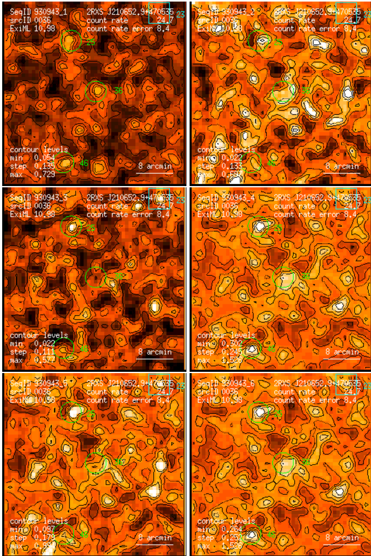
Figure 36: RASS 930943: detection 0036: band rate images, Gaussian filter: (1) PSPC channels 11 – 41, (2) 52 – 90, (3) 91 – 201, (4) 11 – 235, (5) 52 – 201, (6) 11 – 201. Broad band rates in counts/ks. Band rate contour levels in counts/ks/arcmin 2 .
