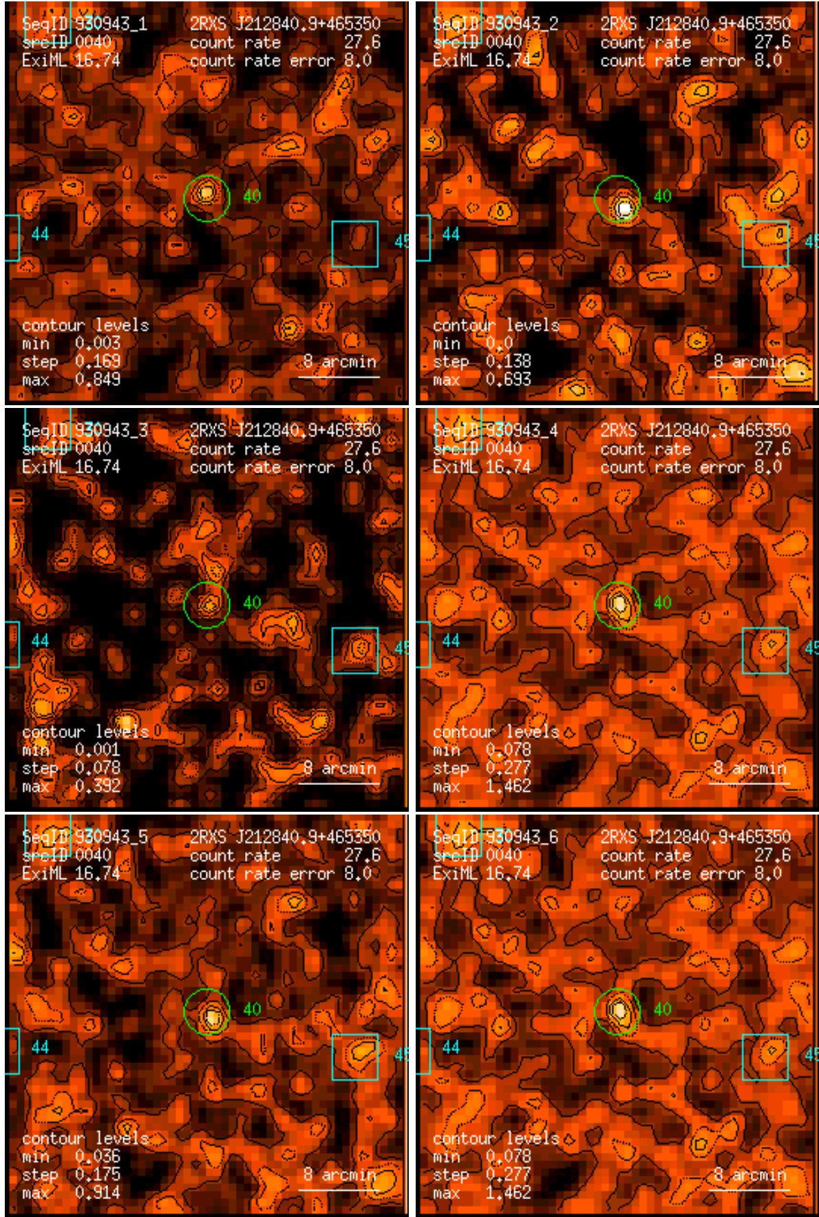
Figure 40: RASS 930943: detection 0040: band rate images, Gaussian filter: (1) PSPC channels 11 – 41, (2) 52 – 90, (3) 91 – 201, (4) 11 – 235, (5) 52 – 201, (6) 11 – 201. Broad band rates in counts/ks. Band rate contour levels in counts/ks/arcmin 2 .
