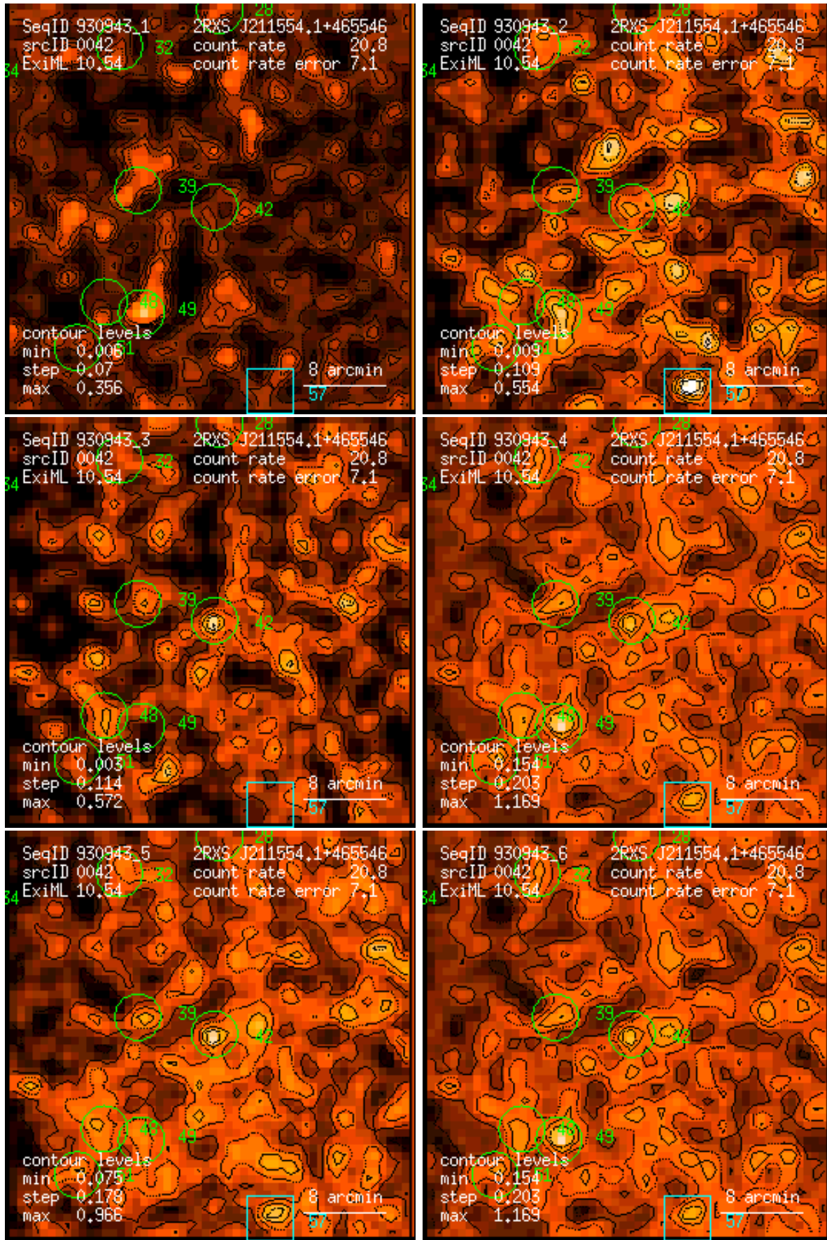
Figure 42: RASS 930943: detection 0042: band rate images, Gaussian filter: (1) PSPC channels 11 – 41, (2) 52 – 90, (3) 91 – 201, (4) 11 – 235, (5) 52 – 201, (6) 11 – 201. Broad band rates in counts/ks. Band rate contour levels in counts/ks/arcmin 2 .
