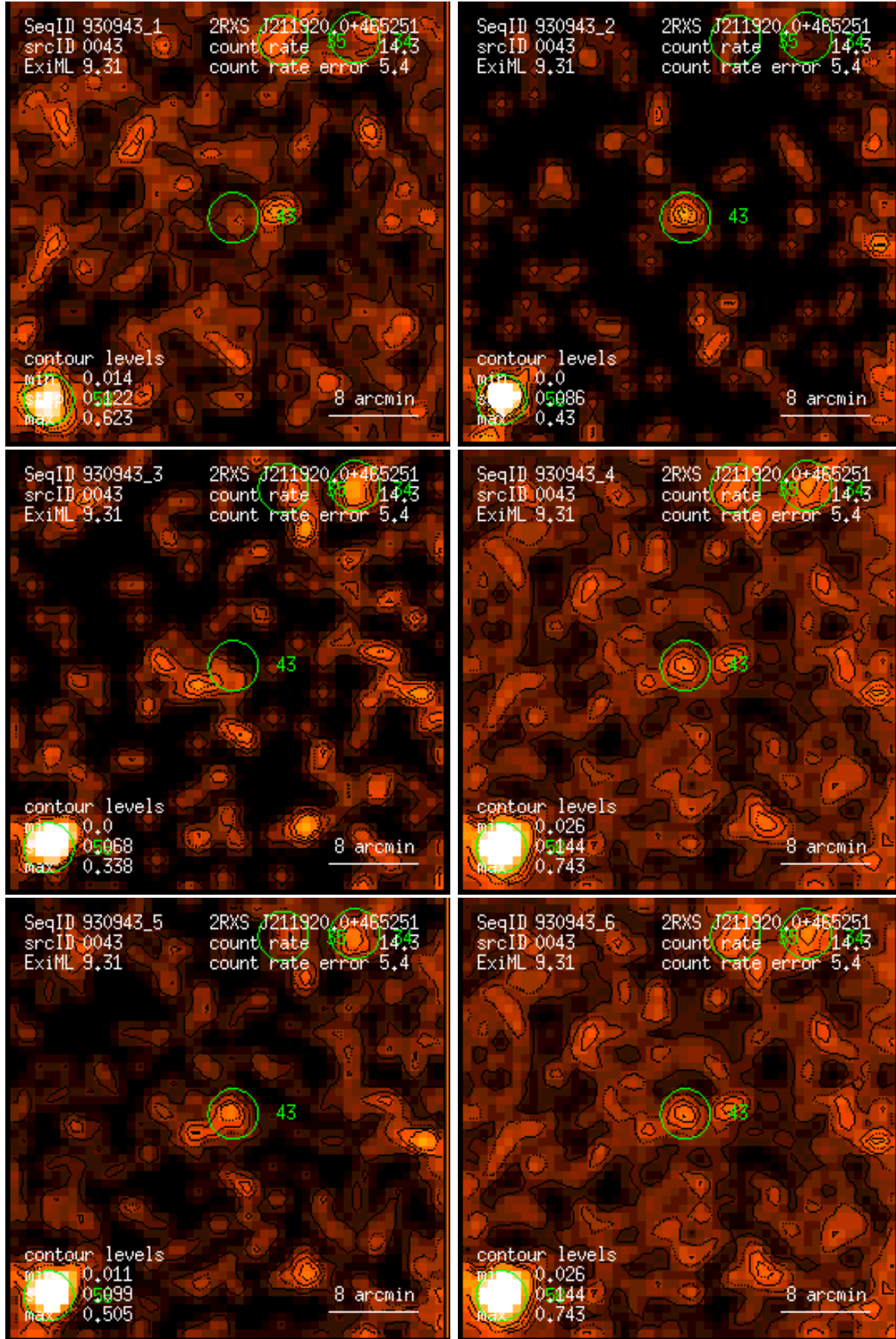
Figure 43: RASS 930943: detection 0043: band rate images, Gaussian filter: (1) PSPC channels 11 – 41, (2) 52 – 90, (3) 91 – 201, (4) 11 – 235, (5) 52 – 201, (6) 11 – 201. Broad band rates in counts/ks. Band rate contour levels in counts/ks/arcmin 2 .
