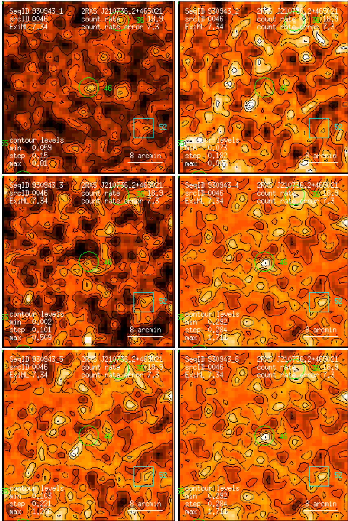
Figure 46: RASS 930943: detection 0046: band rate images, Gaussian filter: (1) PSPC channels 11 – 41, (2) 52 – 90, (3) 91 – 201, (4) 11 – 235, (5) 52 – 201, (6) 11 – 201. Broad band rates in counts/ks. Band rate contour levels in counts/ks/arcmin 2 .
