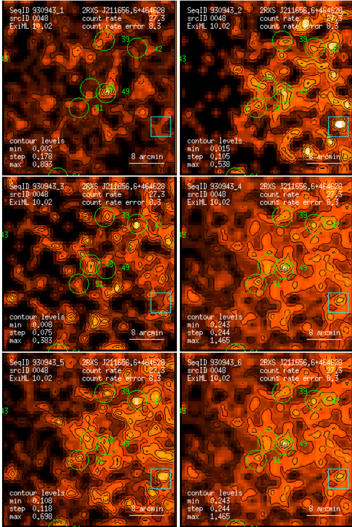
Figure 48: RASS 930943: detection 0048: band rate images, Gaussian filter: (1) PSPC channels 11 – 41, (2) 52 – 90, (3) 91 – 201, (4) 11 – 235, (5) 52 – 201, (6) 11 – 201. Broad band rates in counts/ks. Band rate contour levels in counts/ks/arcmin 2 .
