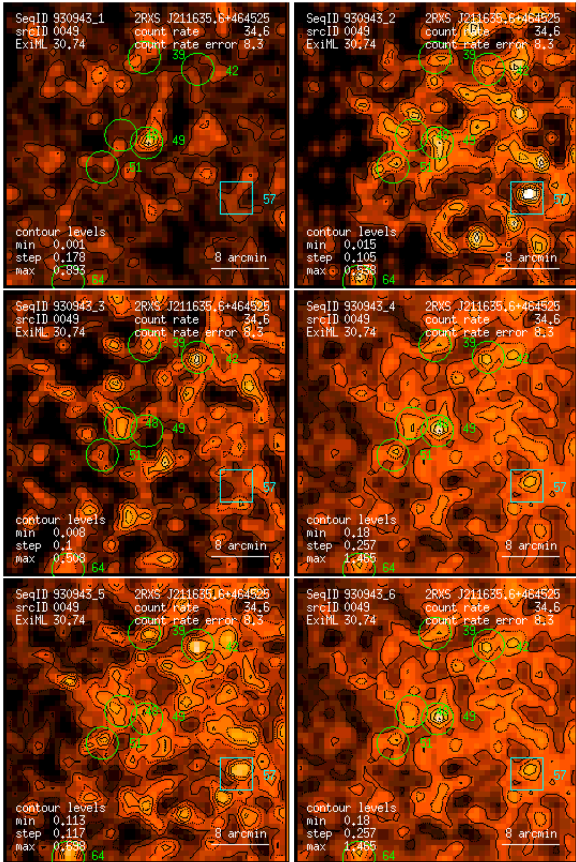
Figure 49: RASS 930943: detection 0049: band rate images, Gaussian filter: (1) PSPC channels 11 – 41, (2) 52 – 90, (3) 91 – 201, (4) 11 – 235, (5) 52 – 201, (6) 11 – 201. Broad band rates in counts/ks. Band rate contour levels in counts/ks/arcmin 2 .
