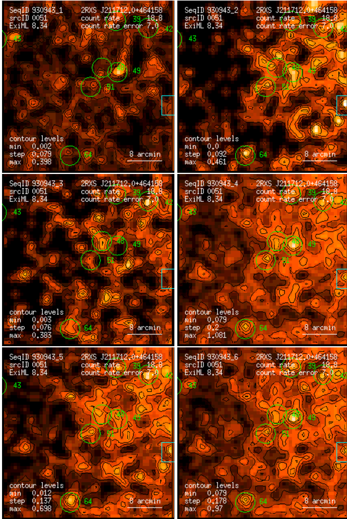
Figure 51: RASS 930943: detection 0051: band rate images, Gaussian filter: (1) PSPC channels 11 – 41, (2) 52 – 90, (3) 91 – 201, (4) 11 – 235, (5) 52 – 201, (6) 11 – 201. Broad band rates in counts/ks. Band rate contour levels in counts/ks/arcmin 2 .
