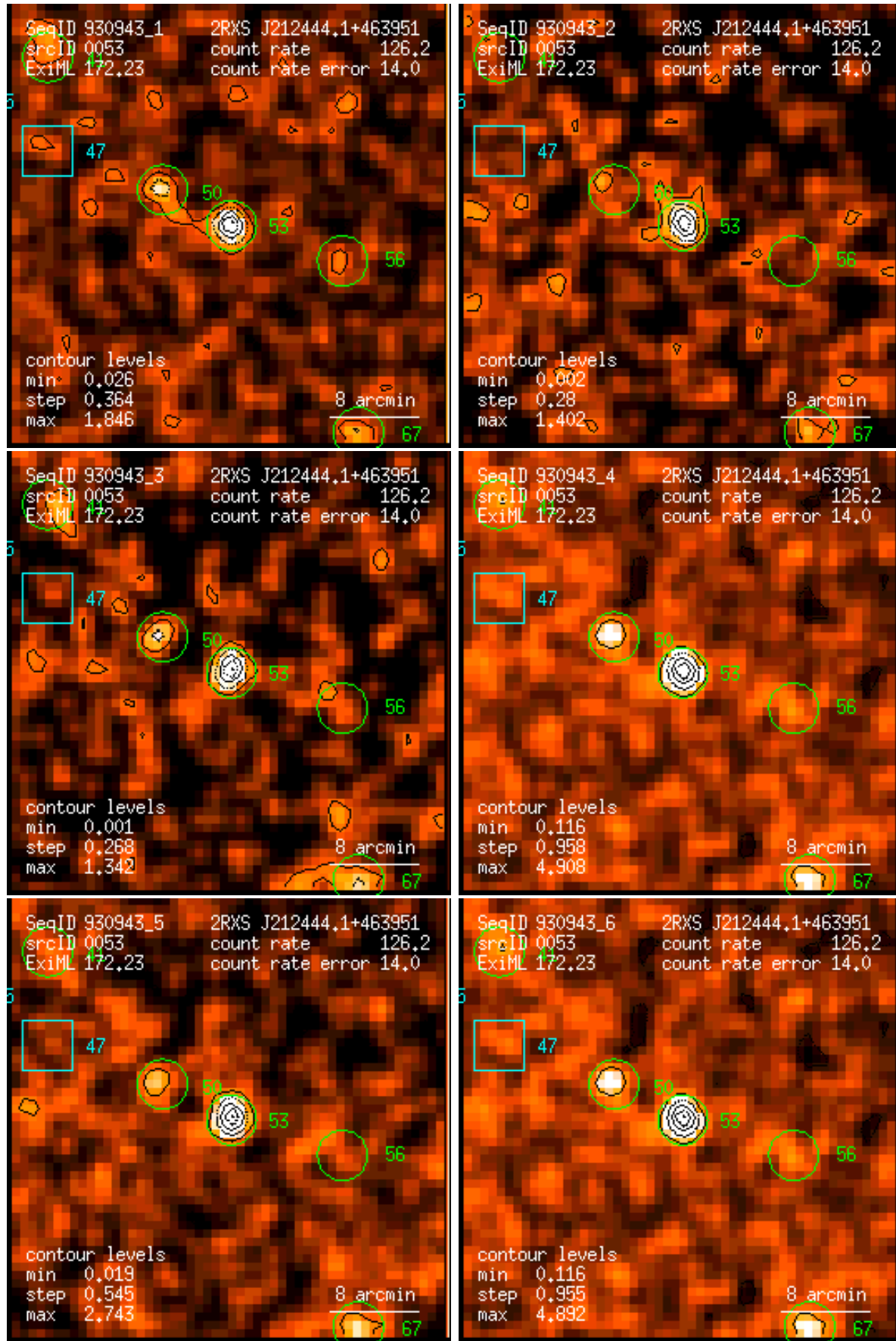
Figure 53: RASS 930943: detection 0053: band rate images, Gaussian filter: (1) PSPC channels 11 – 41, (2) 52 – 90, (3) 91 – 201, (4) 11 – 235, (5) 52 – 201, (6) 11 – 201. Broad band rates in counts/ks. Band rate contour levels in counts/ks/arcmin 2 .
