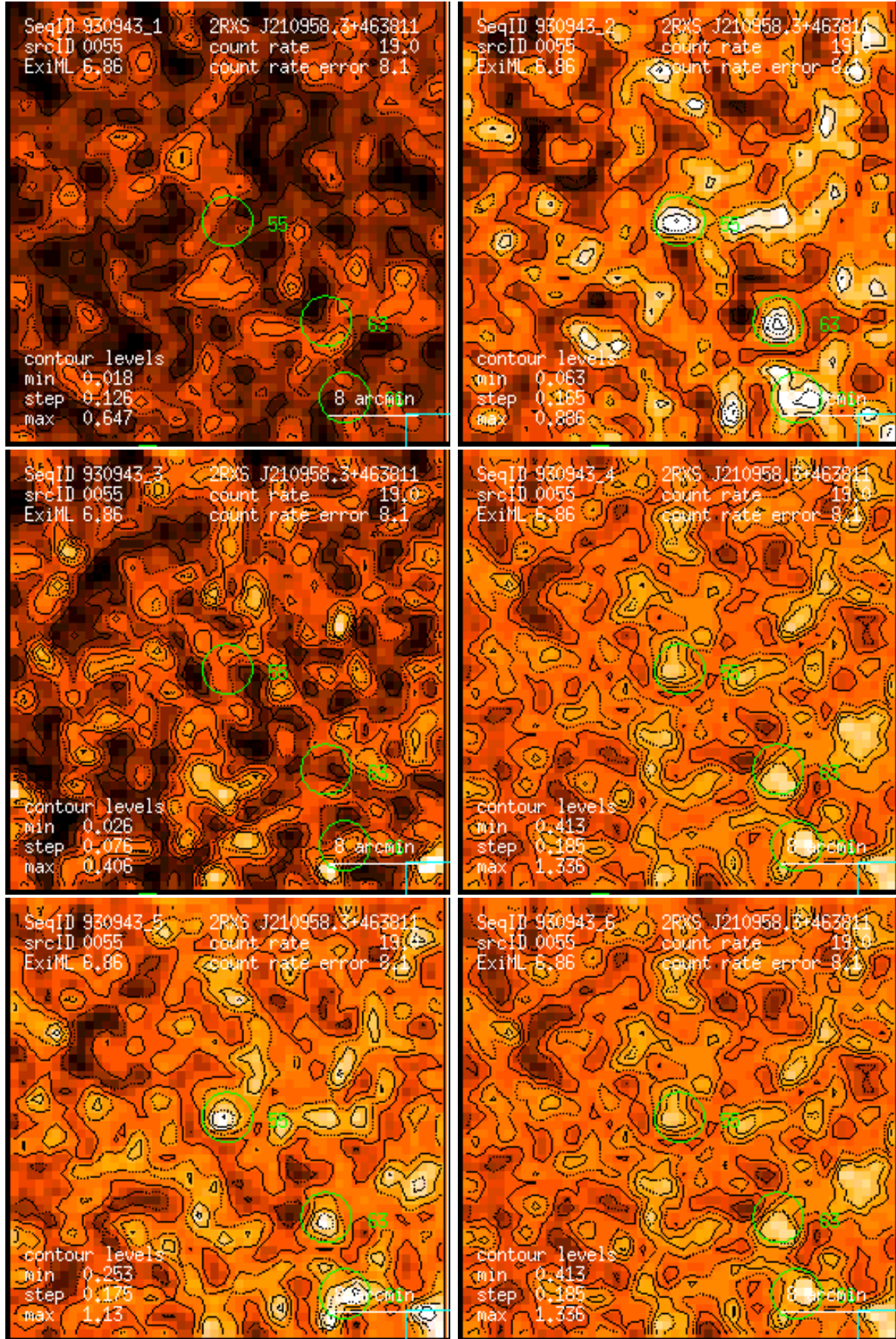
Figure 55: RASS 930943: detection 0055: band rate images, Gaussian filter: (1) PSPC channels 11 – 41, (2) 52 – 90, (3) 91 – 201, (4) 11 – 235, (5) 52 – 201, (6) 11 – 201. Broad band rates in counts/ks. Band rate contour levels in counts/ks/arcmin 2 .
