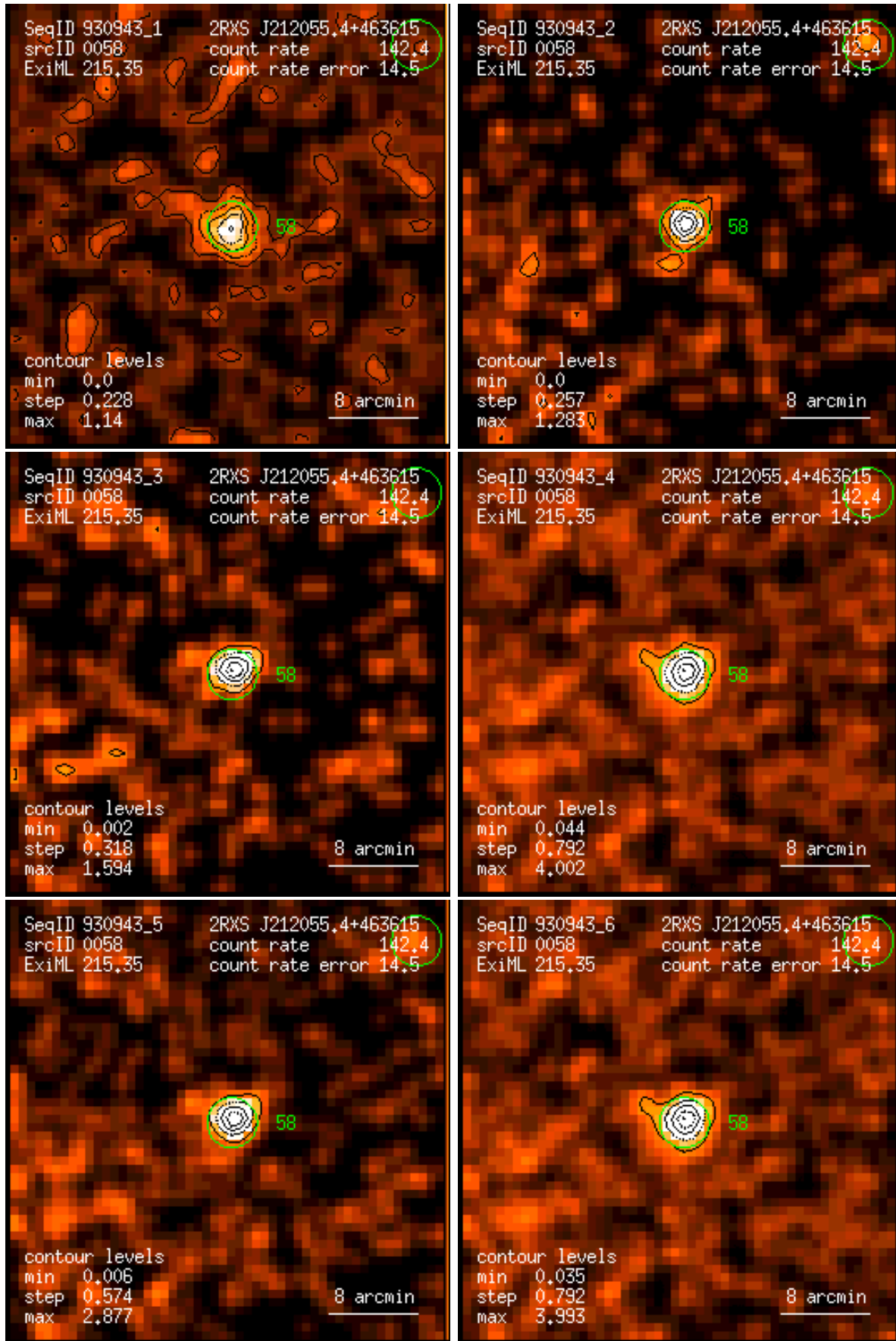
Figure 58: RASS 930943: detection 0058: band rate images, Gaussian filter: (1) PSPC channels 11 – 41, (2) 52 – 90, (3) 91 – 201, (4) 11 – 235, (5) 52 – 201, (6) 11 – 201. Broad band rates in counts/ks. Band rate contour levels in counts/ks/arcmin 2 .
