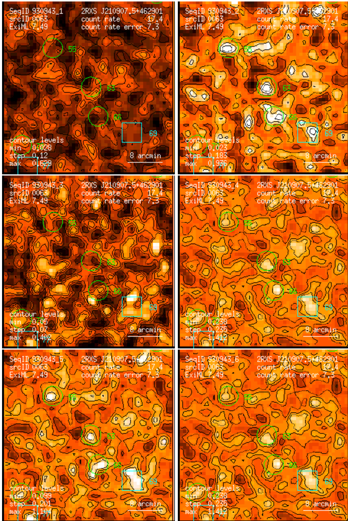
Figure 63: RASS 930943: detection 0063: band rate images, Gaussian filter: (1) PSPC channels 11 – 41, (2) 52 – 90, (3) 91 – 201, (4) 11 – 235, (5) 52 – 201, (6) 11 – 201. Broad band rates in counts/ks. Band rate contour levels in counts/ks/arcmin 2 .
