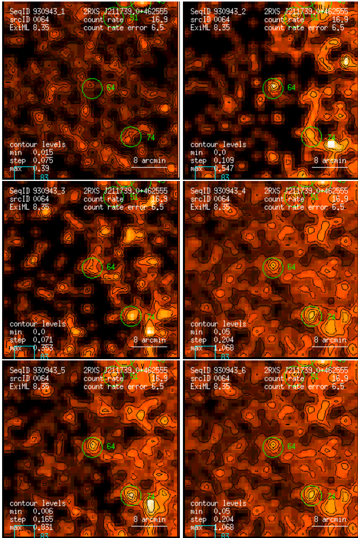
Figure 64: RASS 930943: detection 0064: band rate images, Gaussian filter: (1) PSPC channels 11 – 41, (2) 52 – 90, (3) 91 – 201, (4) 11 – 235, (5) 52 – 201, (6) 11 – 201. Broad band rates in counts/ks. Band rate contour levels in counts/ks/arcmin 2 .
