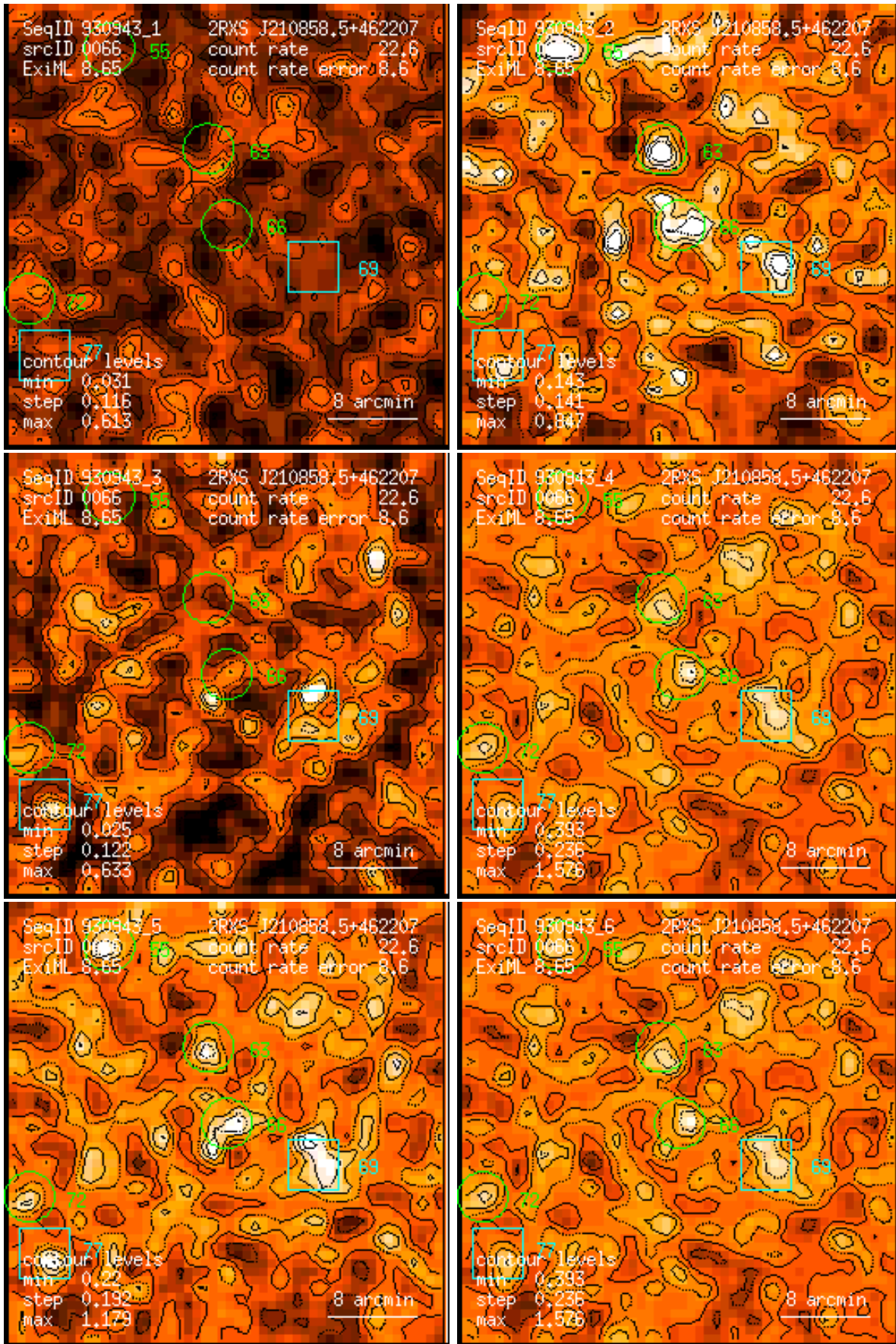
Figure 66: RASS 930943: detection 0066: band rate images, Gaussian filter: (1) PSPC channels 11 – 41, (2) 52 – 90, (3) 91 – 201, (4) 11 – 235, (5) 52 – 201, (6) 11 – 201. Broad band rates in counts/ks. Band rate contour levels in counts/ks/arcmin 2 .
