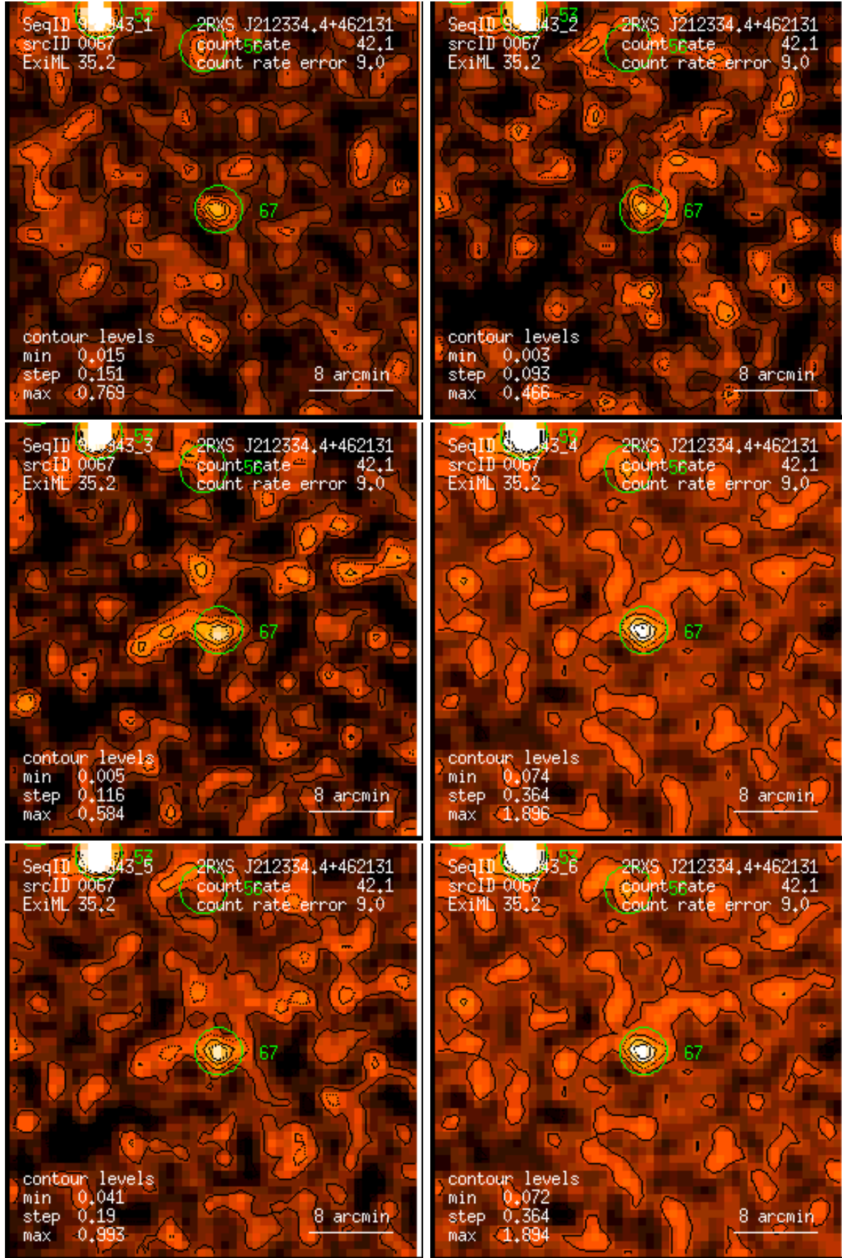
Figure 67: RASS 930943: detection 0067: band rate images, Gaussian filter: (1) PSPC channels 11 – 41, (2) 52 – 90, (3) 91 – 201, (4) 11 – 235, (5) 52 – 201, (6) 11 – 201. Broad band rates in counts/ks. Band rate contour levels in counts/ks/arcmin 2 .
