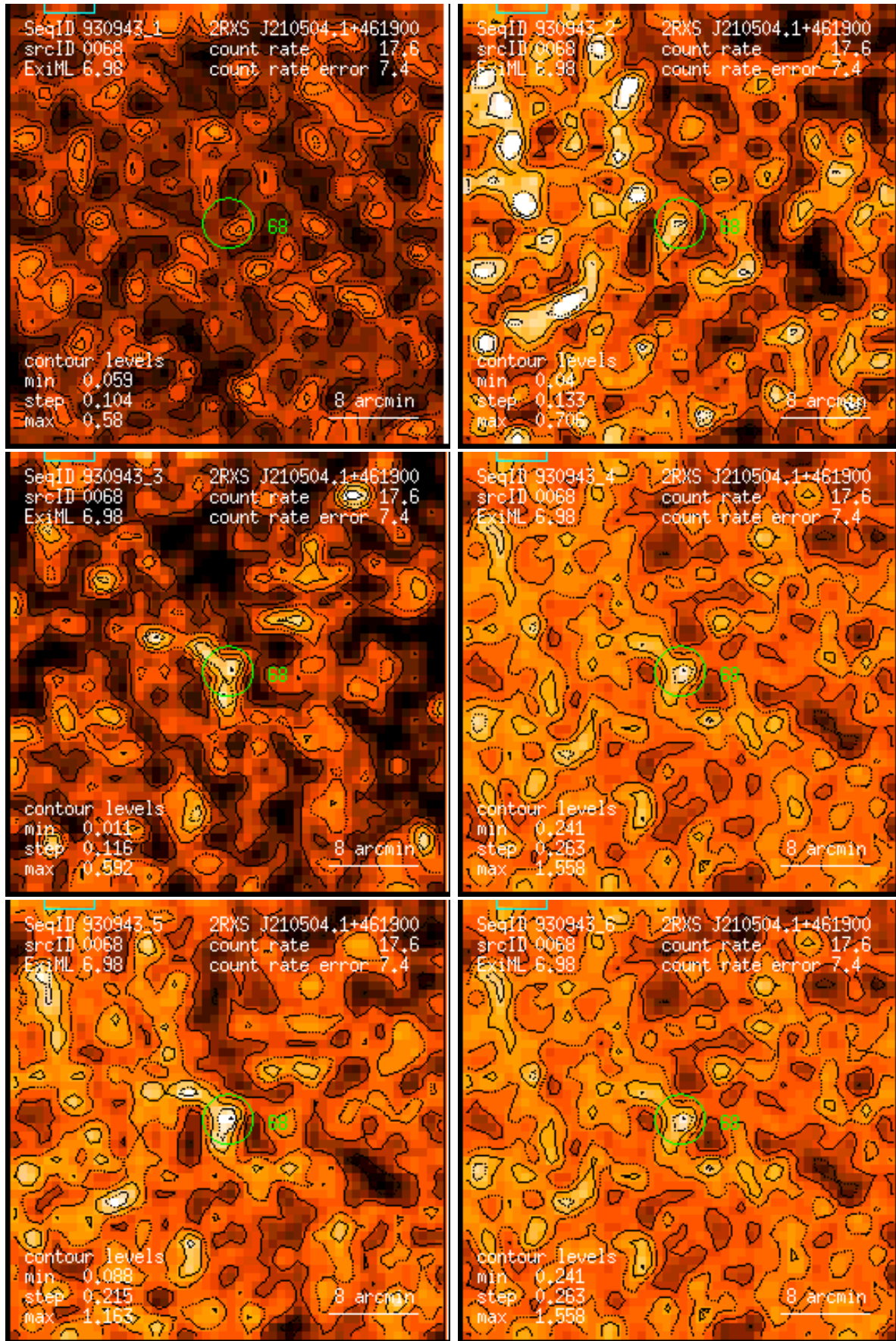
Figure 68: RASS 930943: detection 0068: band rate images, Gaussian filter: (1) PSPC channels 11 – 41, (2) 52 – 90, (3) 91 – 201, (4) 11 – 235, (5) 52 – 201, (6) 11 – 201. Broad band rates in counts/ks. Band rate contour levels in counts/ks/arcmin 2 .
