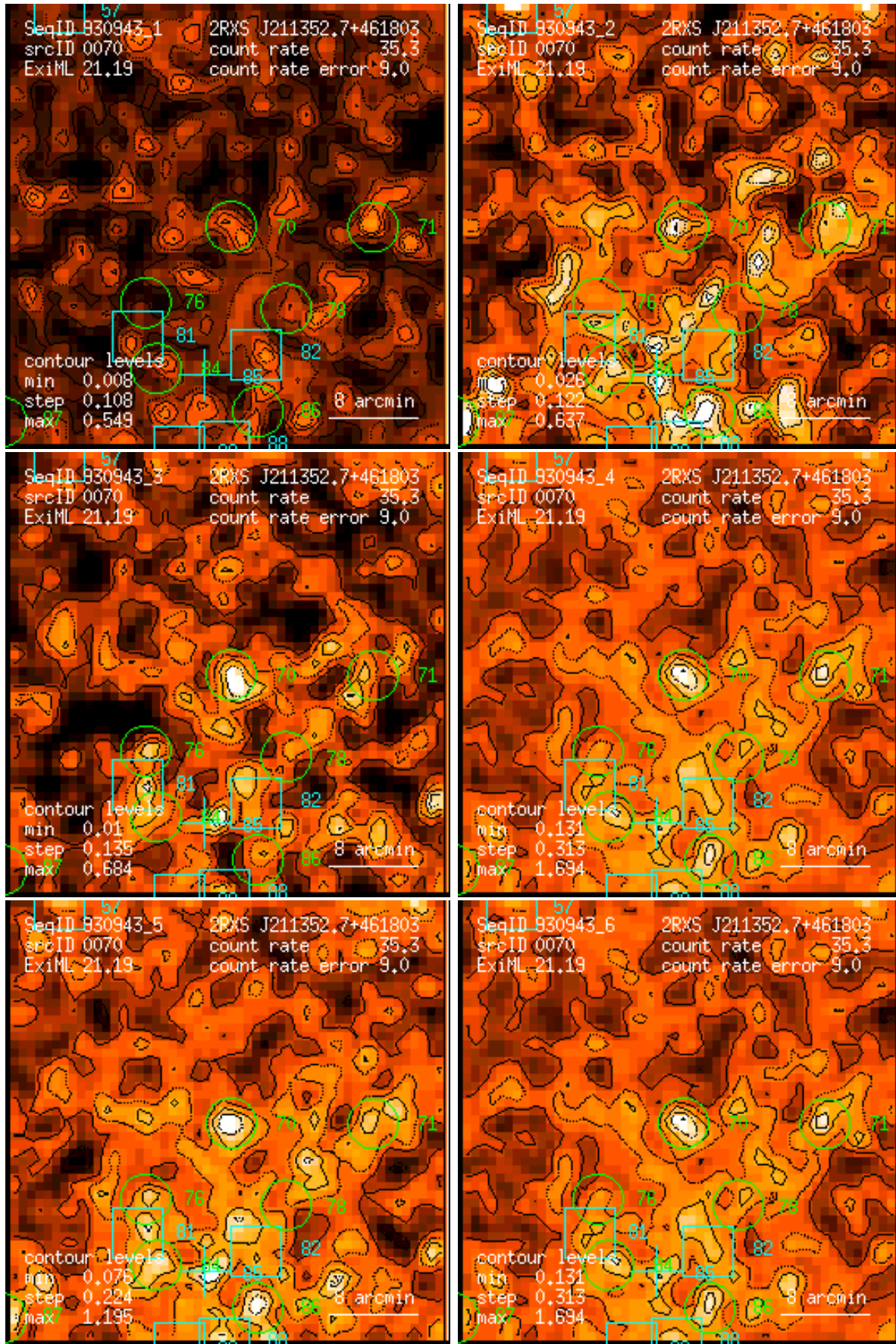
Figure 70: RASS 930943: detection 0070: band rate images, Gaussian filter: (1) PSPC channels 11 – 41, (2) 52 – 90, (3) 91 – 201, (4) 11 – 235, (5) 52 – 201, (6) 11 – 201. Broad band rates in counts/ks. Band rate contour levels in counts/ks/arcmin 2 .
