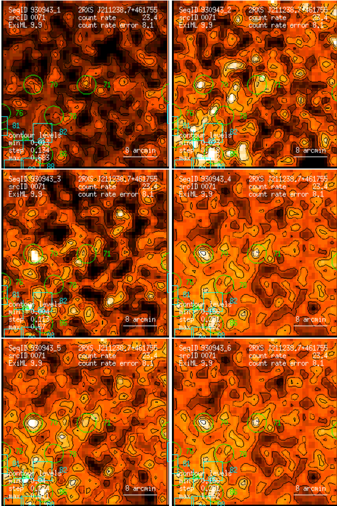
Figure 71: RASS 930943: detection 0071: band rate images, Gaussian filter: (1) PSPC channels 11 – 41, (2) 52 – 90, (3) 91 – 201, (4) 11 – 235, (5) 52 – 201, (6) 11 – 201. Broad band rates in counts/ks. Band rate contour levels in counts/ks/arcmin 2 .
