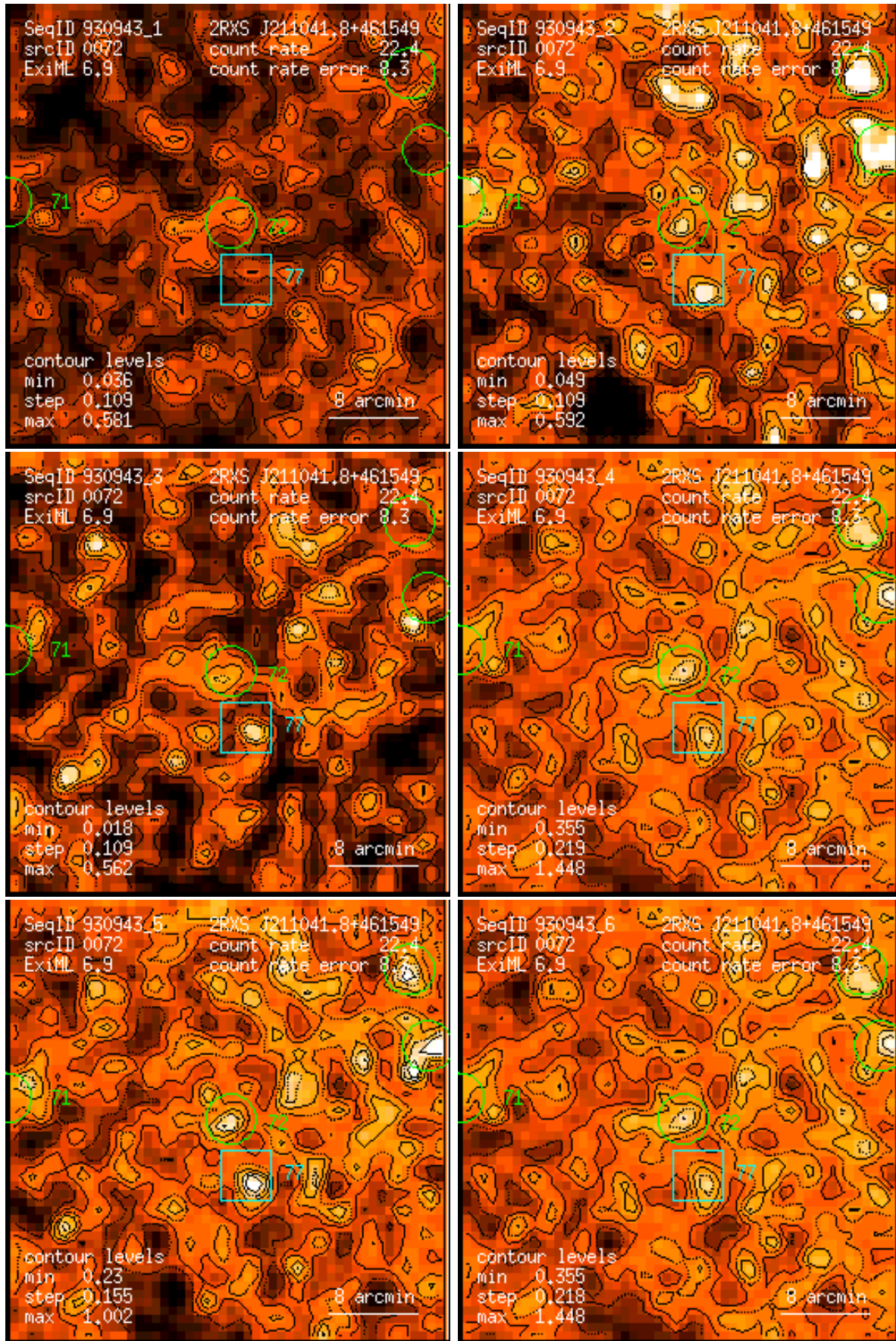
Figure 72: RASS 930943: detection 0072: band rate images, Gaussian filter: (1) PSPC channels 11 – 41, (2) 52 – 90, (3) 91 – 201, (4) 11 – 235, (5) 52 – 201, (6) 11 – 201. Broad band rates in counts/ks. Band rate contour levels in counts/ks/arcmin 2 .
